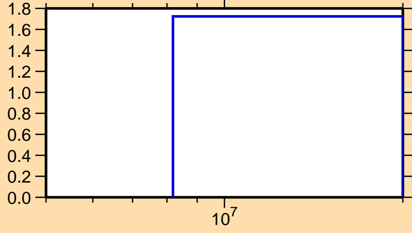
\sigma vs. E for ^{217}\text{Pb}(n,n\alpha)
