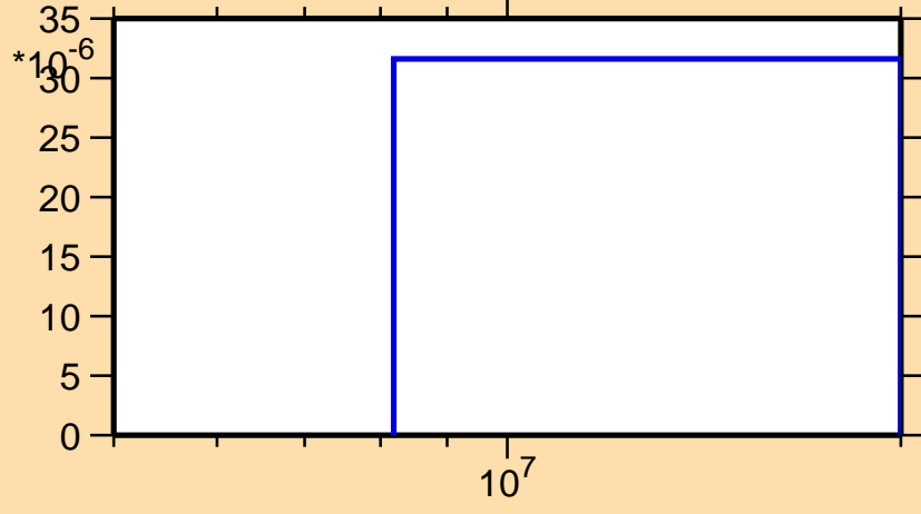
\sigma vs. E for ^{217}\text{Pb}(n,t)
