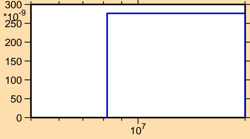
\sigma vs. E for ^{217}\text{Pb}(n,np)
