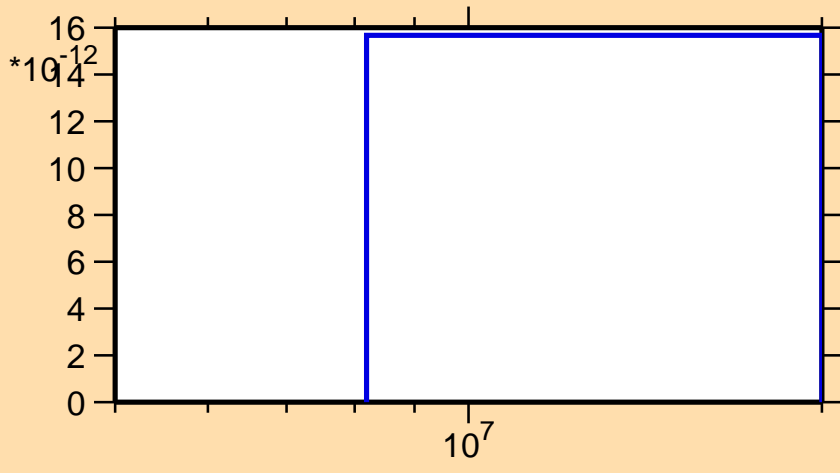
\sigma vs. E for ^{217}\text{Pb}(n,2np)
