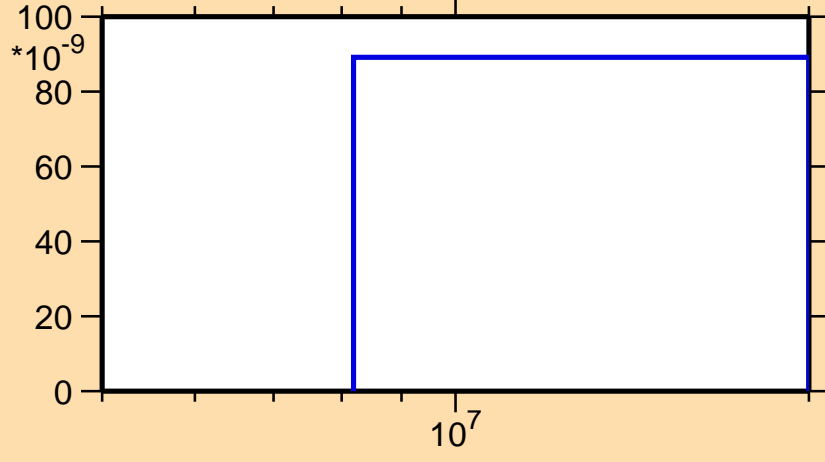
\sigma vs. E for ^{217}\text{Pb}(n,3n\alpha)
