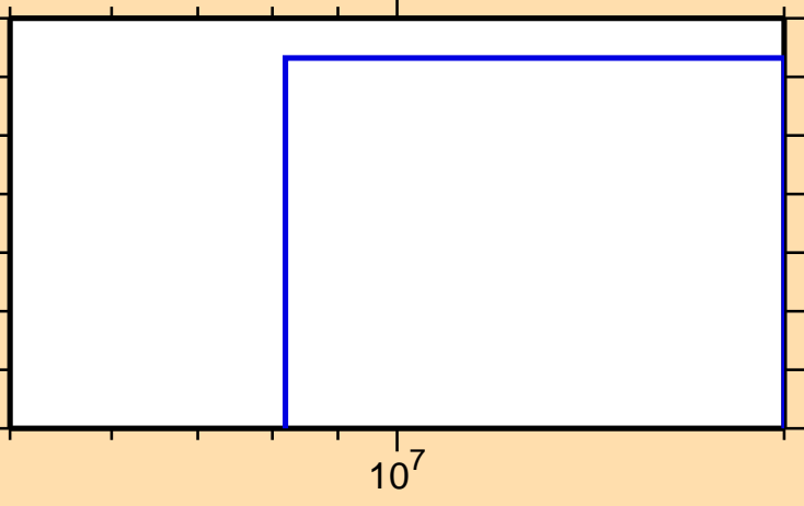
\sigma vs. E for ^{217}\text{Pb}(n,t)
