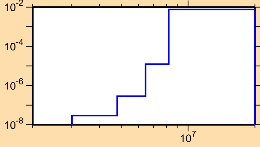
\sigma vs. E for ^{217}\text{Pb}(n,\alpha)
