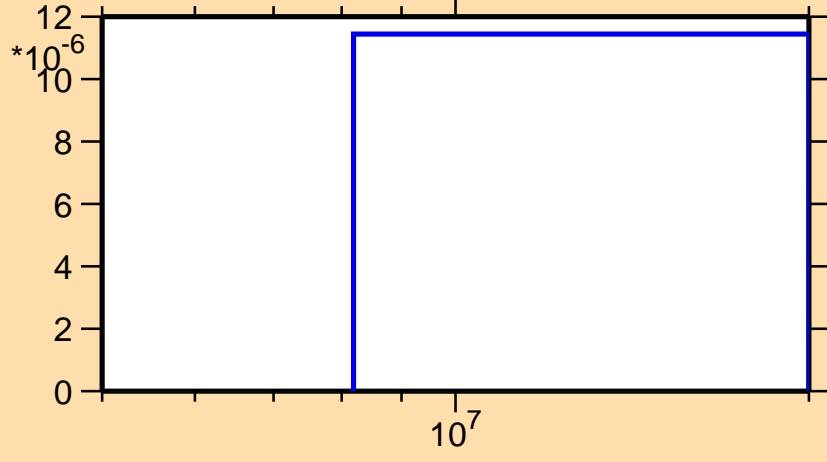
\sigma vs. E for ^{217}\text{Pb}(n,d)
