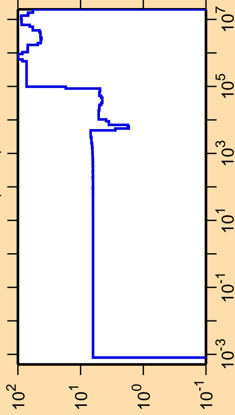
\Delta\sigma/\sigma vs. E for ^{218}\text{Pb}(n,\text{el.})
