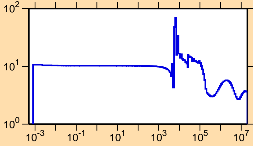
\sigma vs. E for ^{218}\text{Pb}(n,\text{el.})
