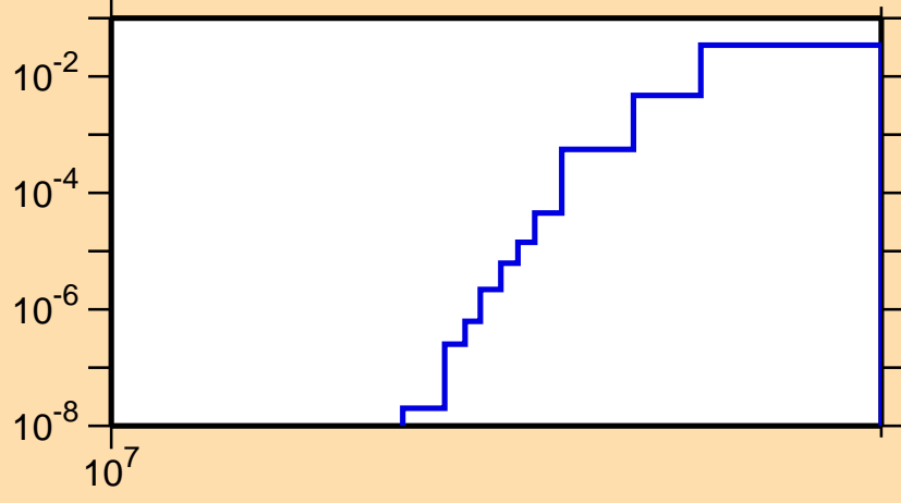
\sigma vs. E for ^{218}\text{Pb}(n,nt)
