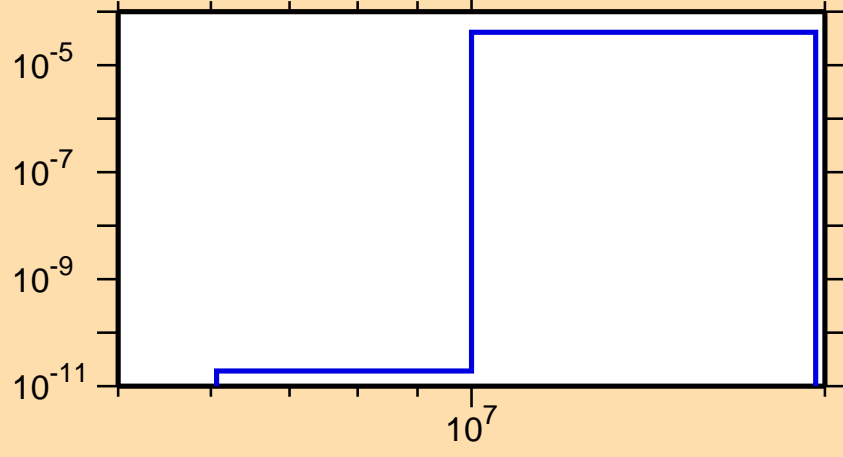
\sigma vs. E for ^{218}\text{Pb}(n,\alpha)
