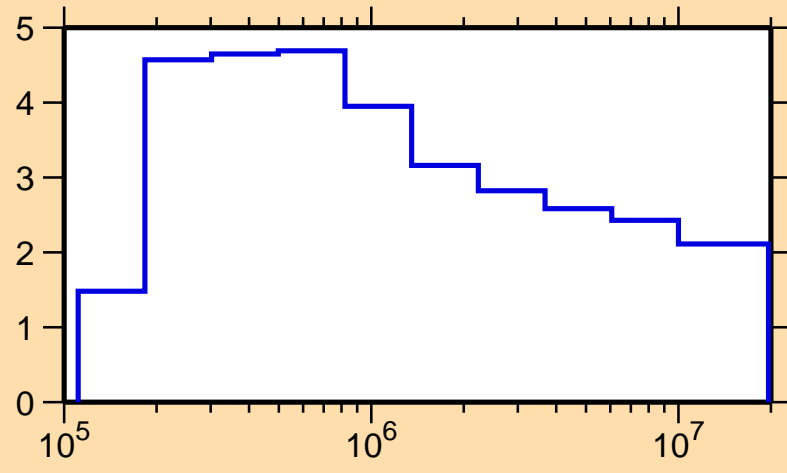
\sigma vs. E for ^{218}\text{Pb}(n,\text{inel.})
