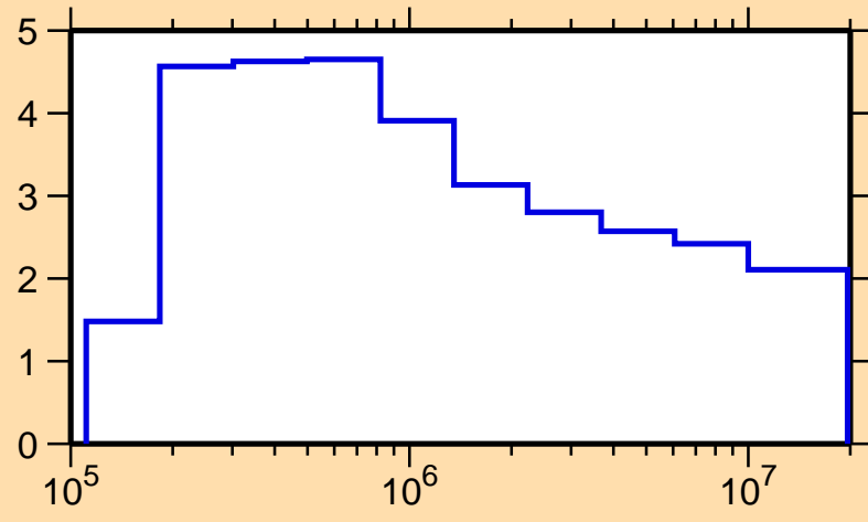
\sigma vs. E for ^{218}\text{Pb}(n,n\text{cont.})
