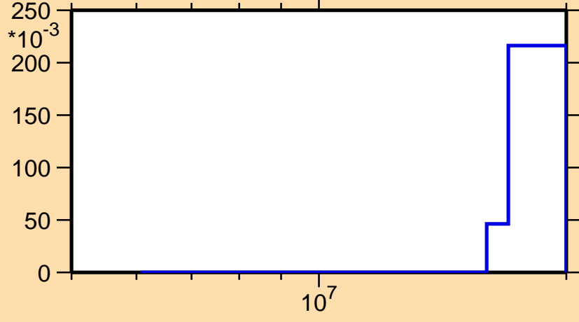
\Delta\sigma/\sigma vs. E for ^{219}\text{Pb}(n,f)
