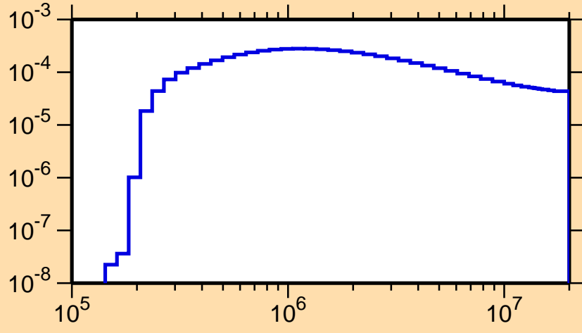
\sigma vs. E for ^{219}\text{Pb}(n,n_1)
