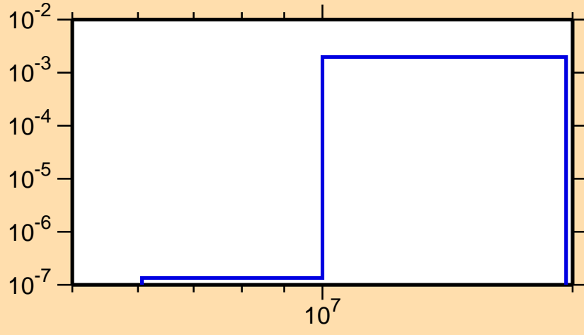
\sigma vs. E for ^{219}\text{Pb}(n,\alpha)
