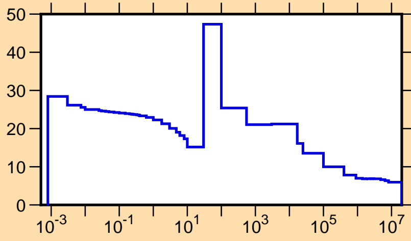
\sigma vs. E for ^{219}\text{Pb}(n,\text{tot.})
