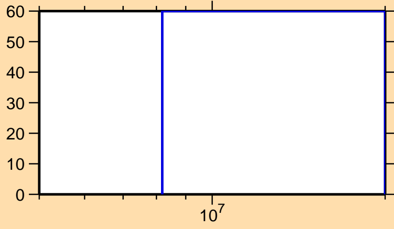
\Delta\sigma/\sigma vs. E for ^{219}\text{Pb}(n,el.)
