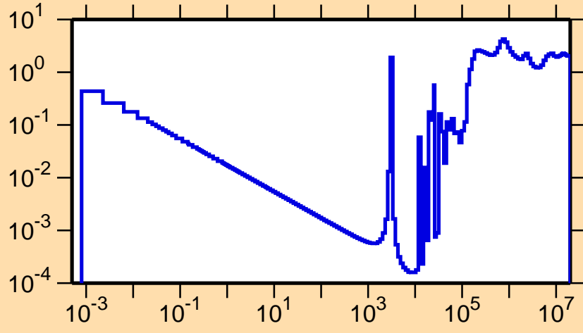
\sigma vs. E for ^{220}\text{Pb}(n,\text{nonel.})
