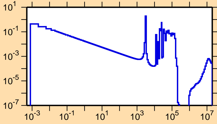
\sigma vs. E for ^{220}\text{Pb}(n,\gamma)
