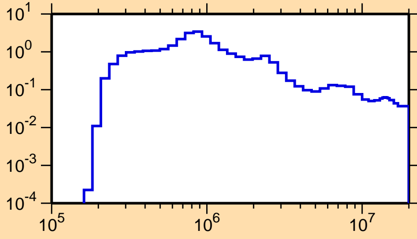
\sigma vs. E for ^{220}\text{Pb}(n,n_1)
