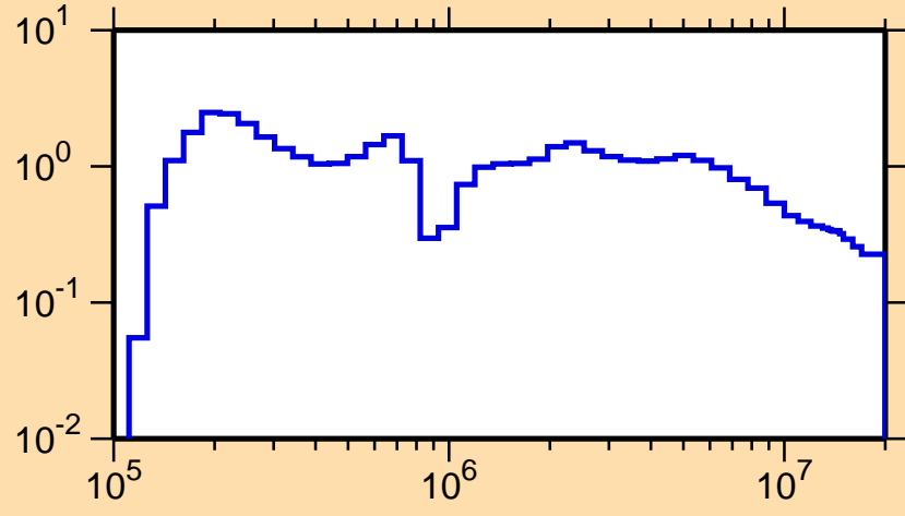
\sigma vs. E for ^{220}\text{Pb}(n,n\text{cont.})
