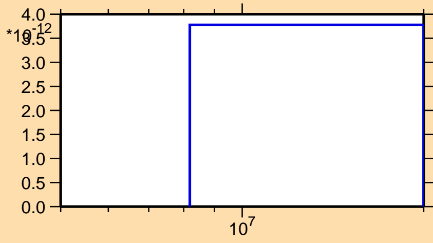
\sigma vs. E for ^{220}\text{Pb}(n,2np)
