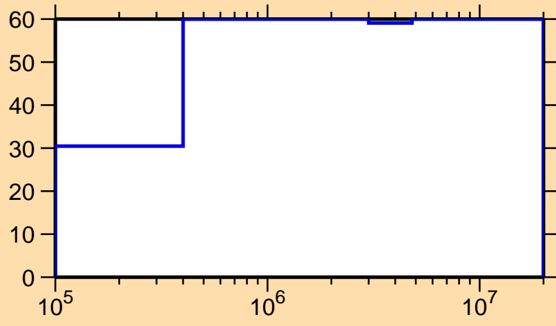
\Delta\sigma/\sigma vs. E for ^{220}\text{Pb}(n,\text{el.})
