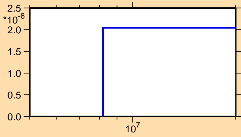
\sigma vs. E for ^{220}\text{Pb}(n,p)
