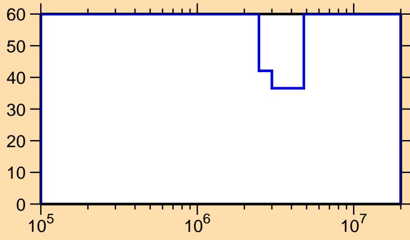
\Delta\sigma/\sigma vs. E for ^{220}\text{Pb}(n,\text{tot.})
