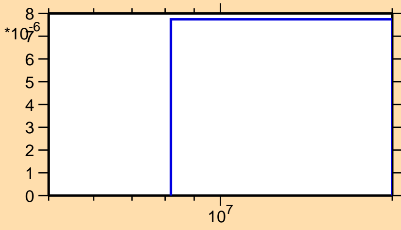
\sigma vs. E for ^{220}\text{Pb}(n,d)
