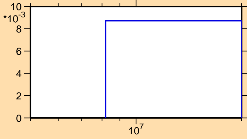
\sigma vs. E for ^{220}\text{Pb}(n,n\alpha)
