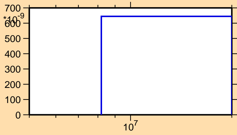
\sigma vs. E for ^{220}\text{Pb}(n,nt)
