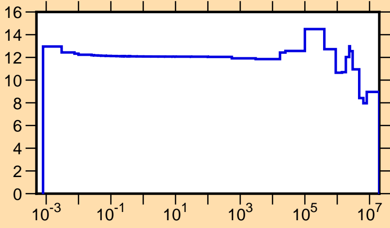
\sigma vs. E for ^{220}\text{Pb}(n,\text{tot.})
