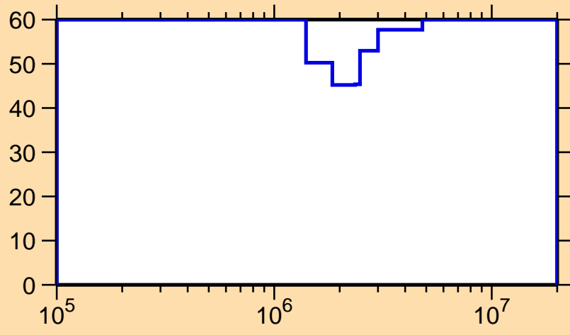
\Delta\sigma/\sigma vs. E for ^{220}\text{Pb}(n,\text{inel.})
