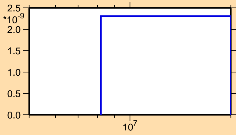
\sigma vs. E for ^{220}\text{Pb}(n,\text{nd})
