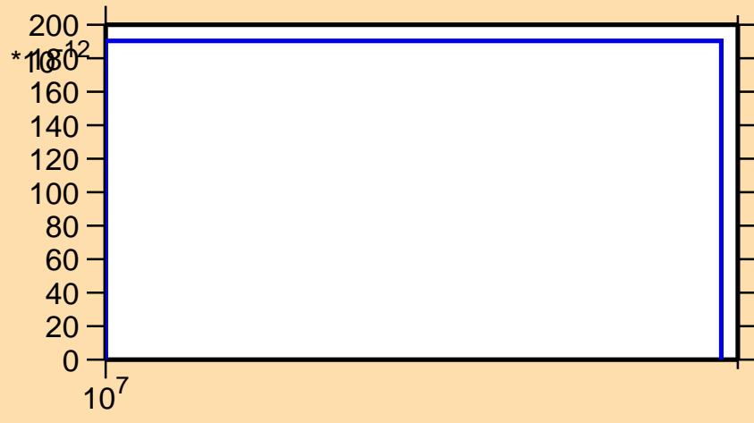
\sigma vs. E for ^{92}\text{Pd}(\text{mt } 45)
