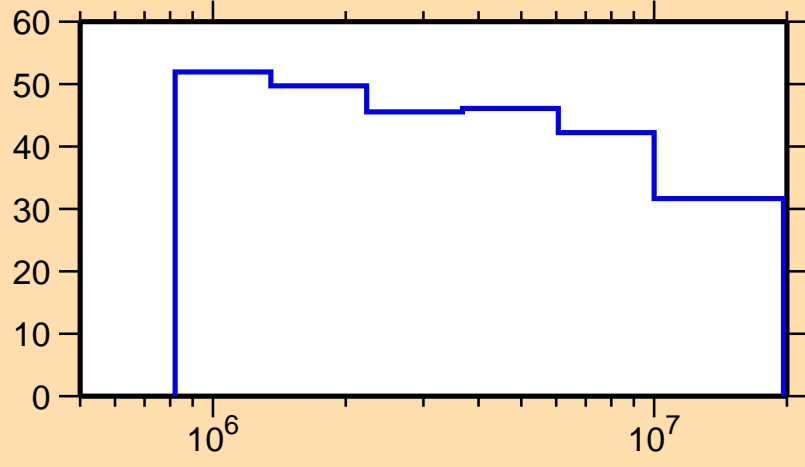
\Delta\sigma/\sigma vs. E for ^{92}\text{Pd}(n,n_1)
