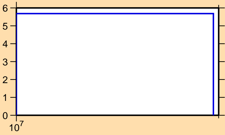
\Delta\sigma/\sigma vs. E for ^{92}\text{Pd}(n,\text{el.})
