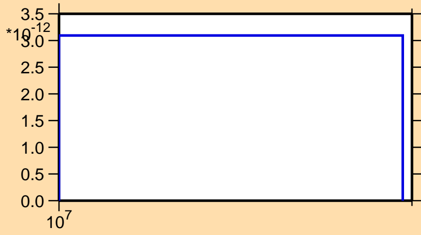
\sigma vs. E for ^{92}\text{Pd}(\text{mt117})
