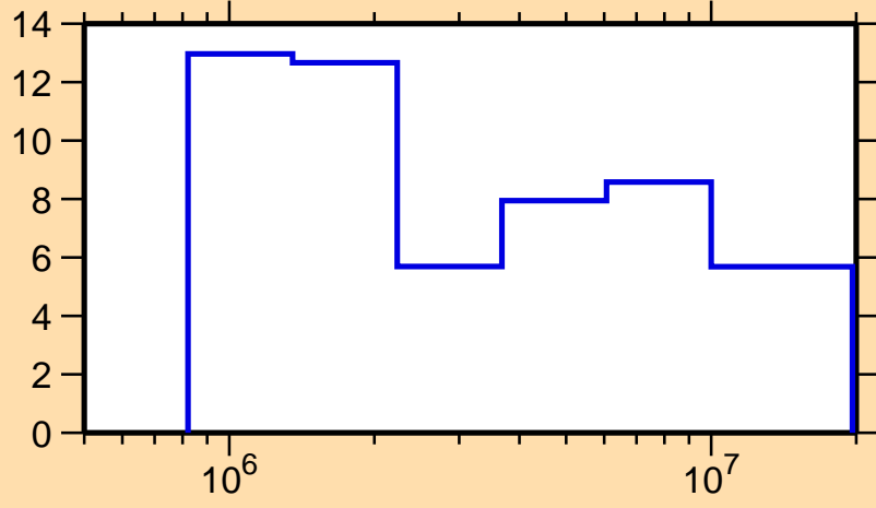
\Delta\sigma/\sigma vs. E for ^{92}\text{Pd}(n,\text{el.})
