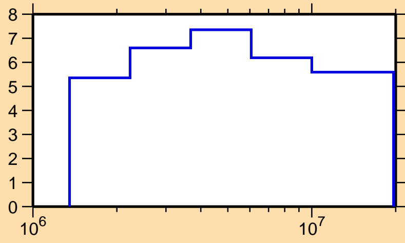
\Delta\sigma/\sigma vs. E for ^{92}\text{Pd}(n,\text{nonel.})
