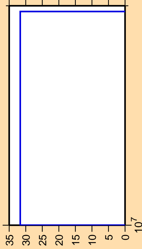
\Delta\sigma/\sigma vs. E for ^{92}\text{Pd}(n,n_1)
