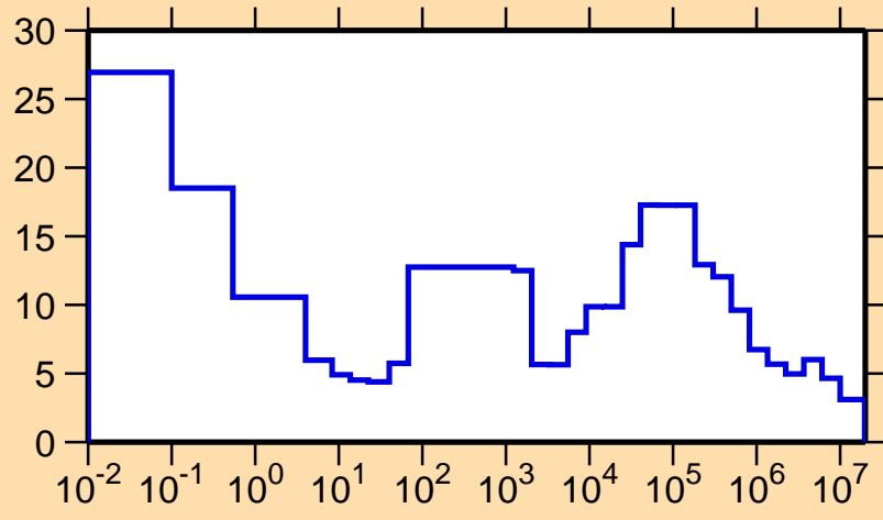
\Delta\sigma/\sigma vs. E for ^{92}\text{Pd}(n,\text{tot.})
