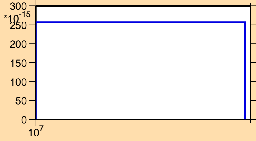
\sigma vs. E for ^{92}\text{Pd}(\text{mt } 34)
