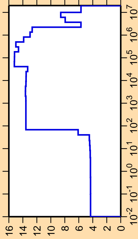
\Delta\sigma/\sigma vs. E for ^{92}\text{Pd}(n,\text{el.})
