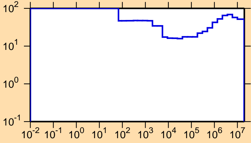
\Delta\sigma/\sigma vs. E for ^{92}\text{Pd}(n,p)
