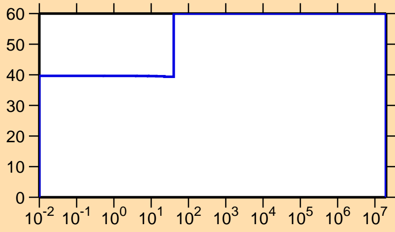
\Delta\sigma/\sigma vs. E for ^{92}\text{Pd}(n,\gamma)
