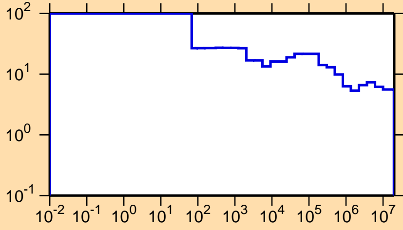
\Delta\sigma/\sigma vs. E for ^{92}\text{Pd}(n,\text{nonel.})
