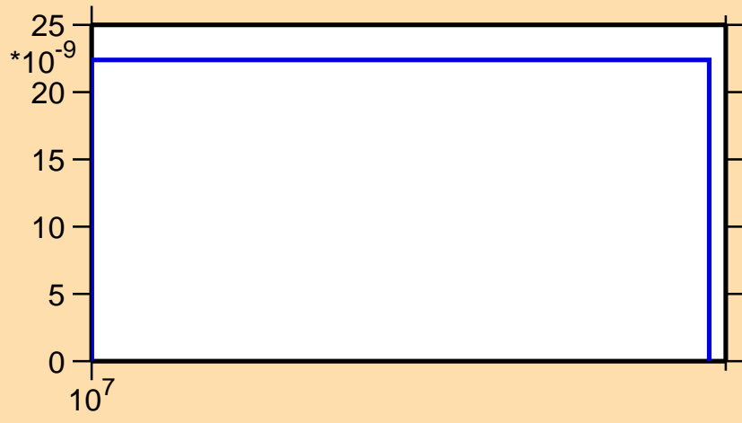
\sigma vs. E for ^{92}\text{Pd}(n,2n)
