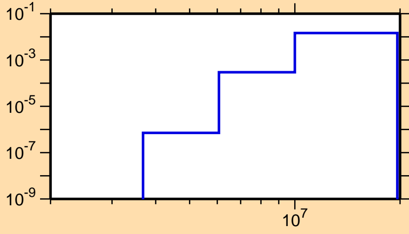
\sigma vs. E for ^{92}\text{Pd}(n,d)
