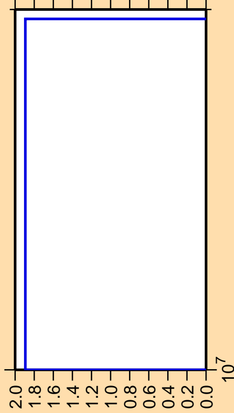
\Delta\sigma/\sigma vs. E for ^{92}\text{Pd}(\text{mt } 34)
