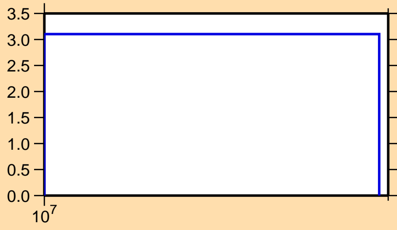
\Delta\sigma/\sigma vs. E for ^{92}\text{Pd}(n,\text{tot.})
