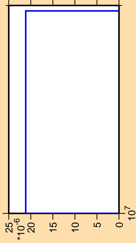
\Delta\sigma/\sigma vs. E for ^{92}\text{Pd}(n,2np)
