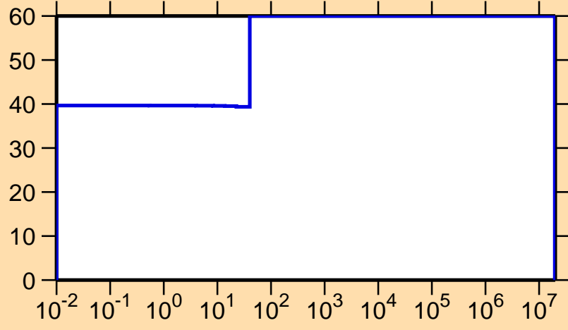
\Delta\sigma/\sigma vs. E for ^{92}\text{Pd}(n,\gamma)
