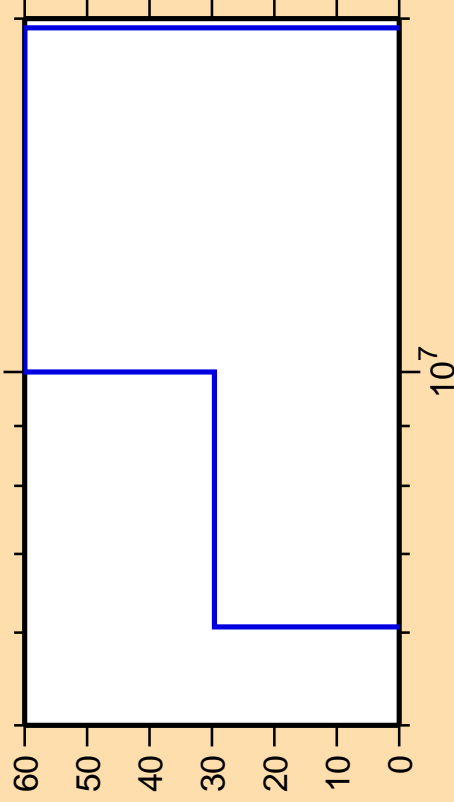
\Delta\sigma/\sigma vs. E for ^{92}\text{Pd}(n,n\alpha)
