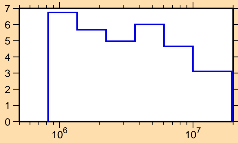
\Delta\sigma/\sigma vs. E for ^{92}\text{Pd}(n,\text{tot.})
