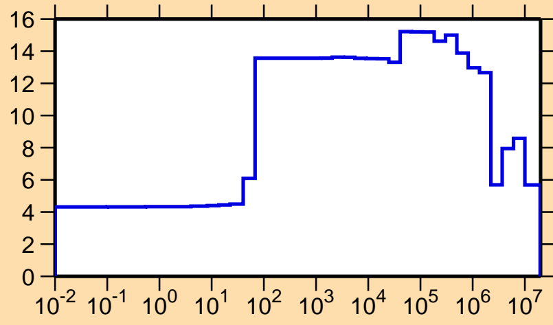
\Delta\sigma/\sigma vs. E for ^{92}\text{Pd}(n,\text{el.})
