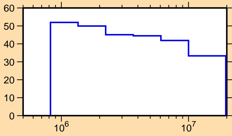
\Delta\sigma/\sigma vs. E for ^{92}\text{Pd}(n,\text{inel.})
