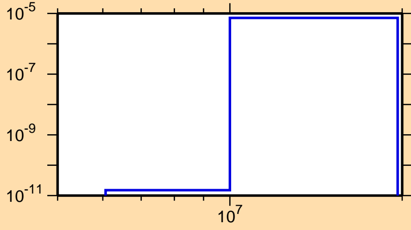
\sigma vs. E for ^{92}\text{Pd}(n,n\alpha)
