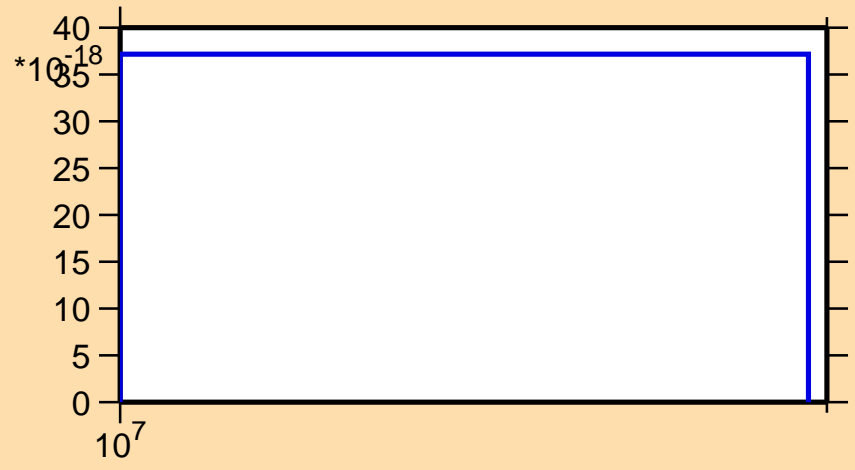
\sigma vs. E for ^{92}\text{Pd}(n,2np)
