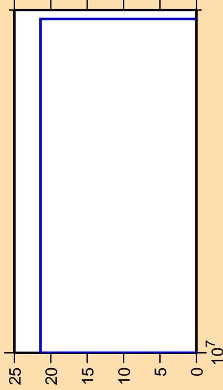
\Delta\sigma/\sigma vs. E for ^{92}\text{Pd}(\text{mt117})
