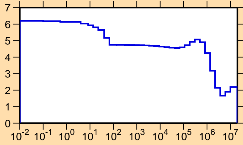
\sigma vs. E for ^{92}\text{Pd}(n,\text{el.})
