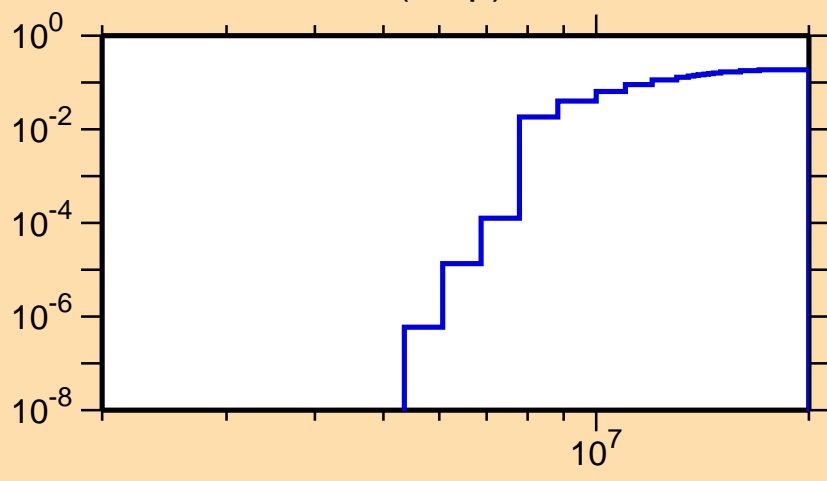
\sigma vs. E for ^{93}\text{Pd}(n,np)
