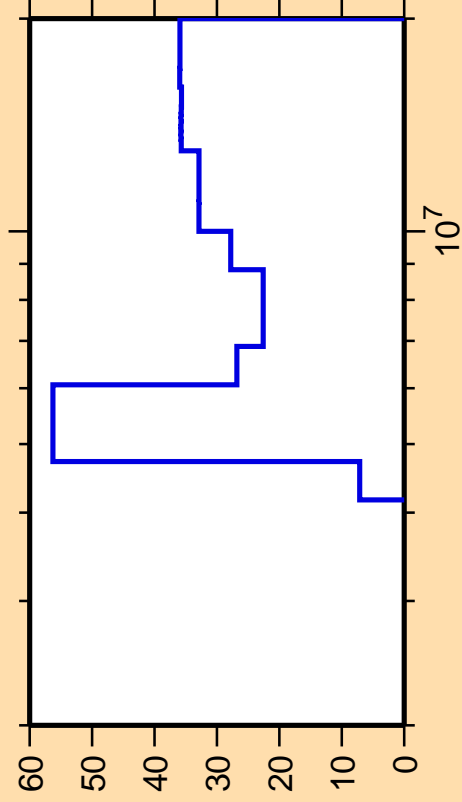
\Delta\sigma/\sigma vs. E for ^{93}\text{Pd}(n,np)
