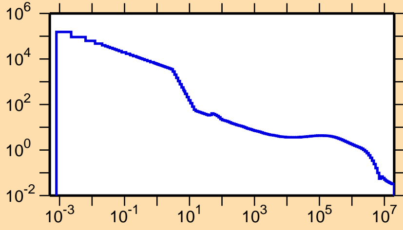
\sigma vs. E for ^{93}\text{Pd}(n,p)
