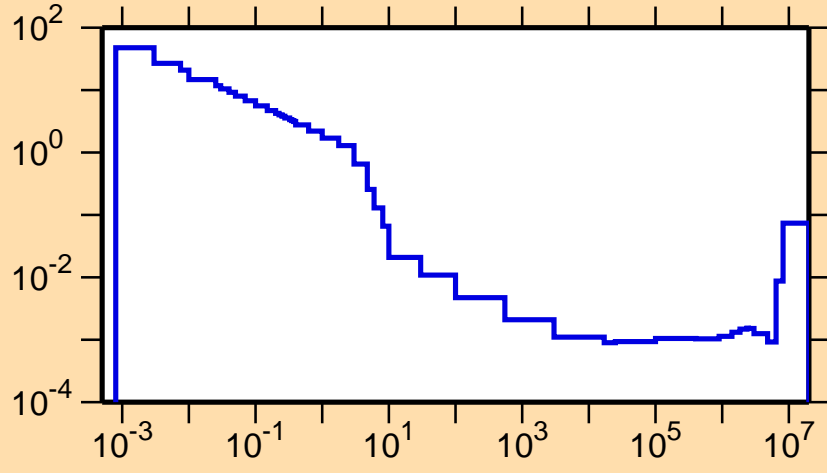
\sigma vs. E for ^{93}\text{Pd}(n,\alpha)
