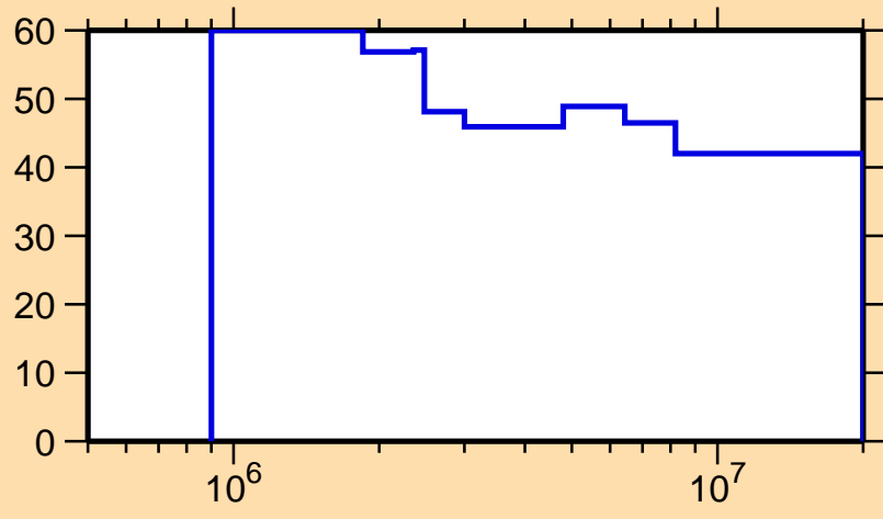
\Delta\sigma/\sigma vs. E for ^{93}\text{Pd}(n,n_1)
