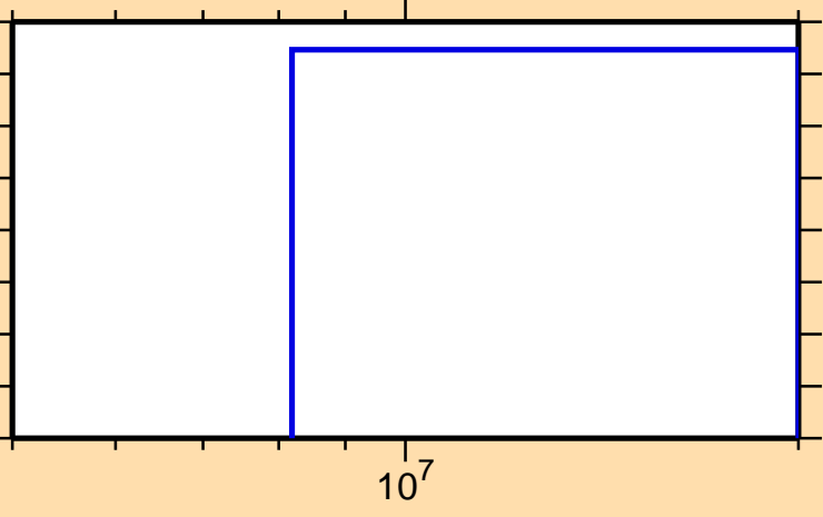
\sigma vs. E for ^{93}\text{Pd}(n,t)
