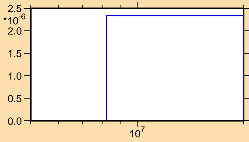
\sigma vs. E for ^{93}\text{Pd}(n,\text{pt})
