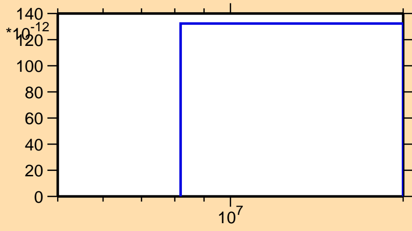
\sigma vs. E for ^{93}\text{Pd}(\text{mt } 34)
