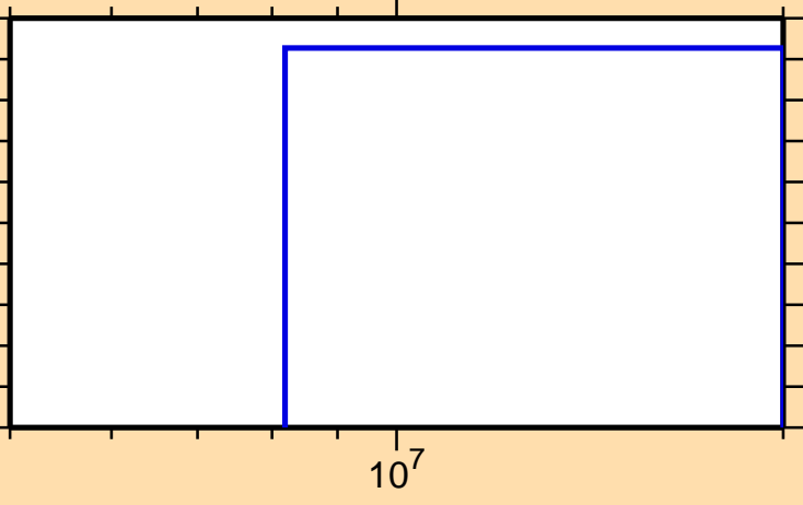
\sigma vs. E for ^{93}\text{Pd}(n,2n)
