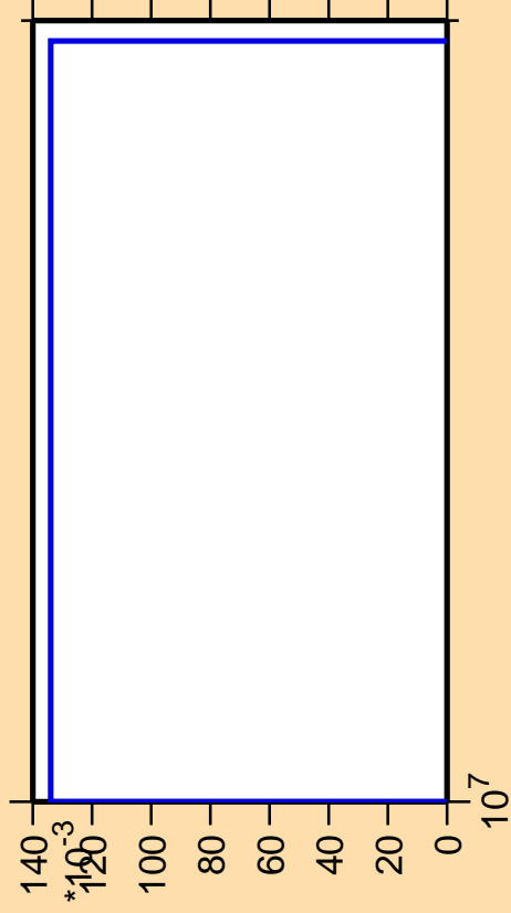
\Delta\sigma/\sigma vs. E for ^{94}\text{Pd}(n,nd)
