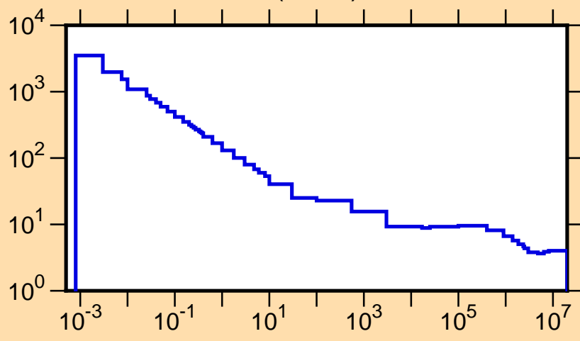
\sigma vs. E for ^{94}\text{Pd}(n,\text{tot.})
