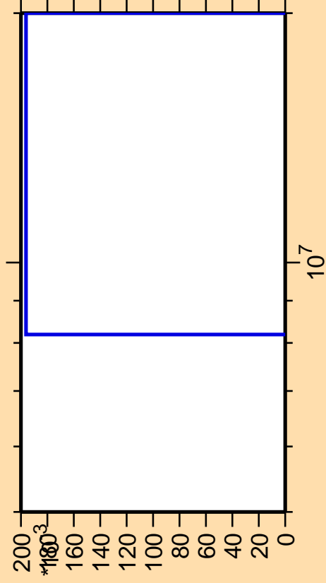
\Delta\sigma/\sigma vs. E for ^{94}\text{Pd}(n,\text{nd})
