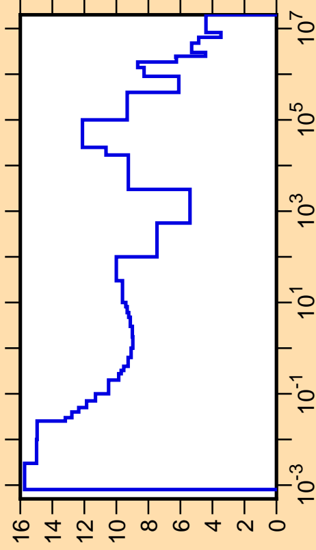
\Delta\sigma/\sigma vs. E for ^{94}\text{Pd}(n,\text{tot.})
