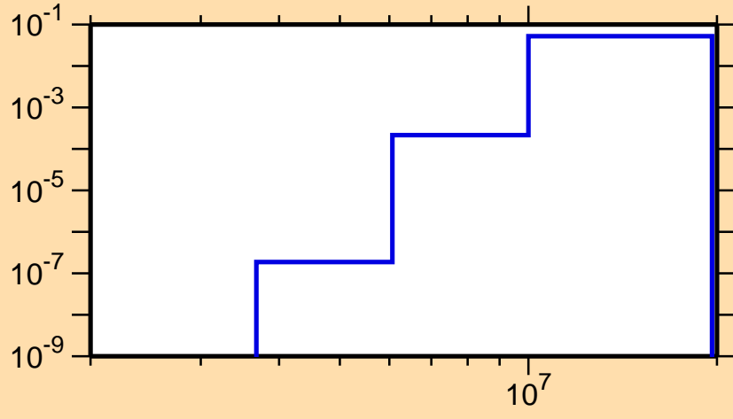
\sigma vs. E for ^{95}\text{Pd}(n,p\alpha)
