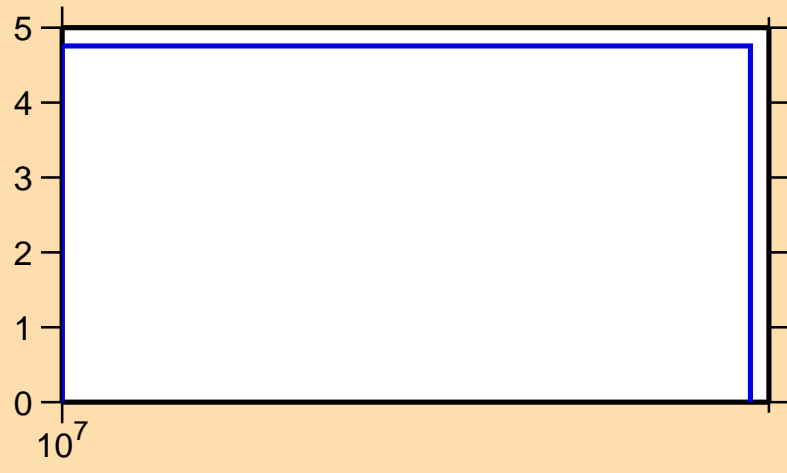
\Delta\sigma/\sigma vs. E for ^{95}\text{Pd}(n,\text{el.})
