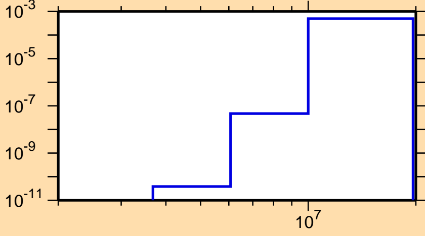
\sigma vs. E for ^{95}\text{Pd}(n,\text{He}3)
