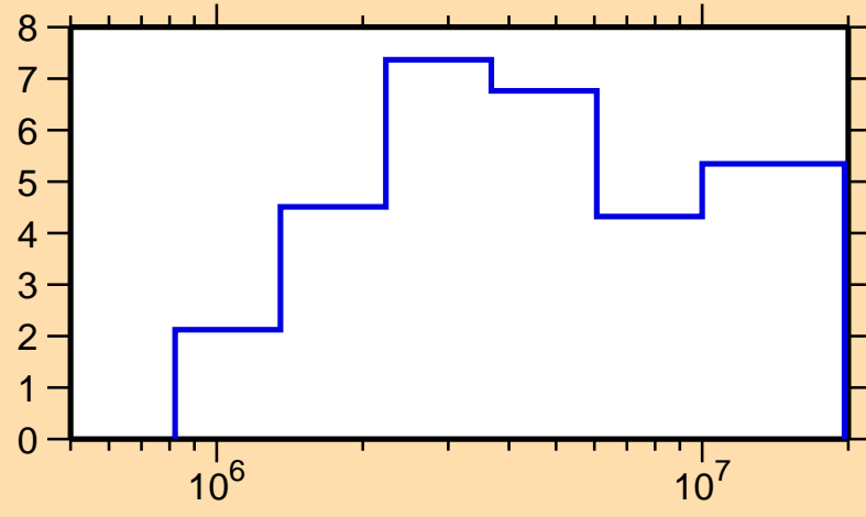
\Delta\sigma/\sigma vs. E for ^{95}\text{Pd}(n,\text{tot.})
