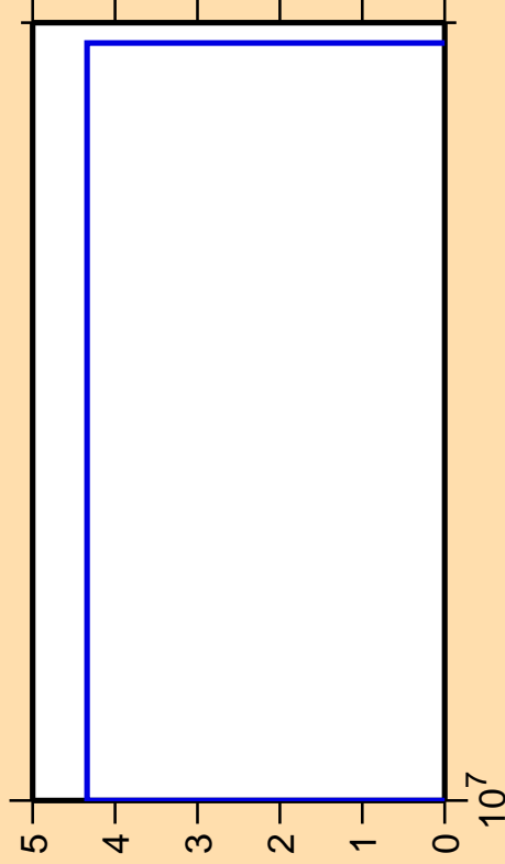
\Delta\sigma/\sigma vs. E for ^{95}\text{Pd}(\text{mt } 45)
