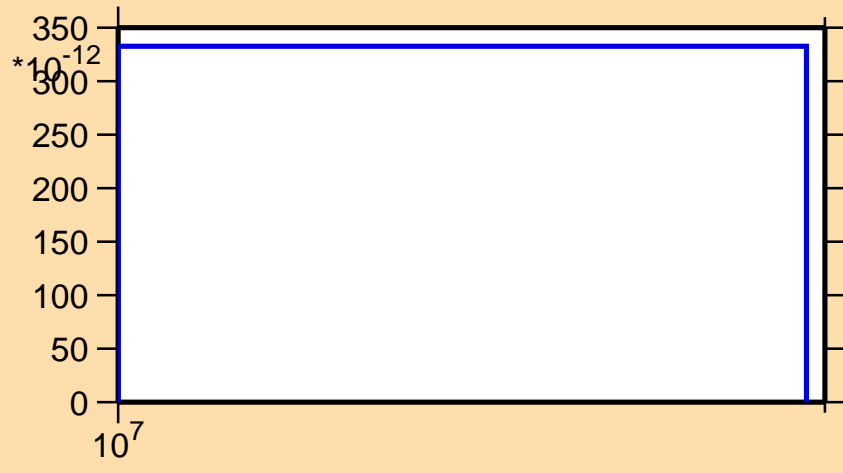
\sigma vs. E for ^{95}\text{Pd}(n,\text{nd})
