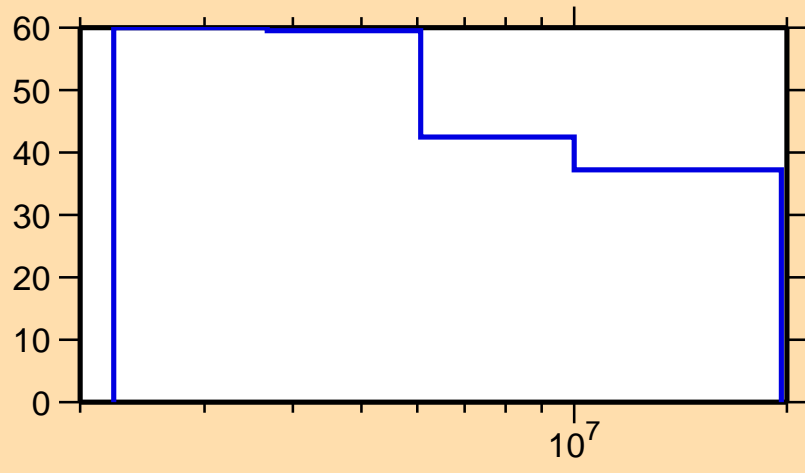
\Delta\sigma/\sigma vs. E for ^{95}\text{Pd}(n,ncont.)
