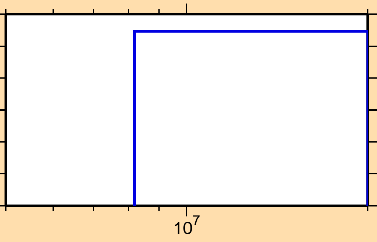
\sigma vs. E for ^{95}\text{Pd}(n,\text{pt})
