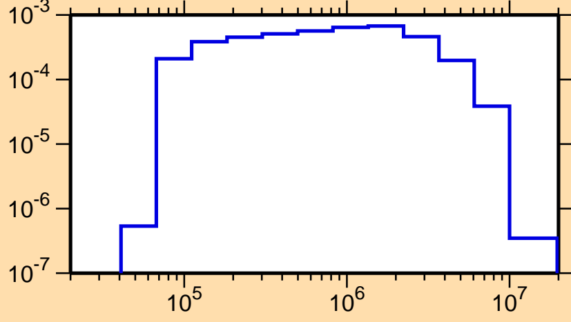
\sigma vs. E for ^{95}\text{Pd}(n,n_2)
