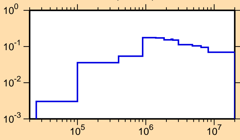
\sigma vs. E for ^{95}\text{Pd}(n,\text{inel.})
