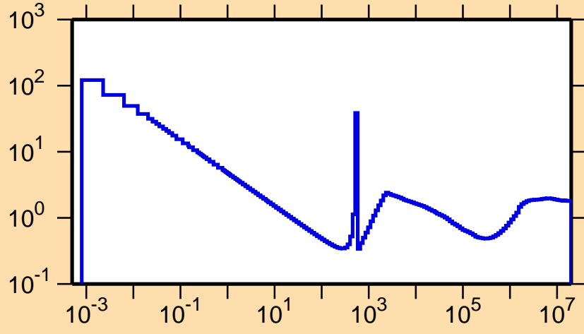
\sigma vs. E for ^{96}\text{Pd}(n,\text{nonel.})
