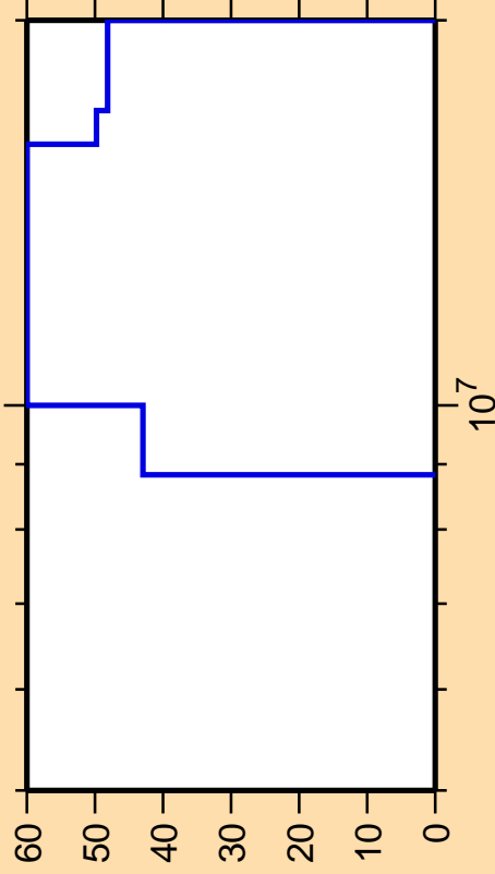
\Delta\sigma/\sigma vs. E for ^{96}\text{Pd}(n,n\alpha)
