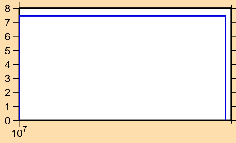
\Delta\sigma/\sigma vs. E for ^{96}\text{Pd}(n,\text{el.})
