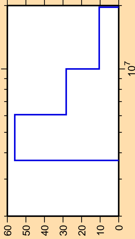
\Delta\sigma/\sigma vs. E for ^{96}\text{Pd}(n,n\text{cont.})
