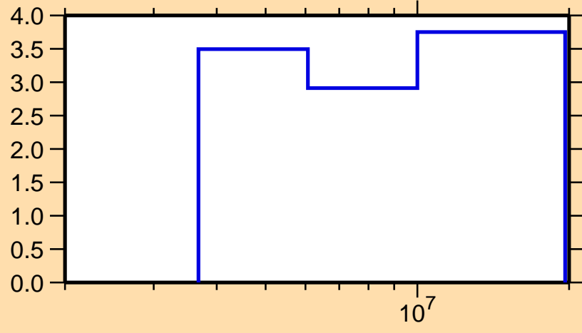
\Delta\sigma/\sigma vs. E for ^{96}\text{Pd}(n,n\text{nonel.})
