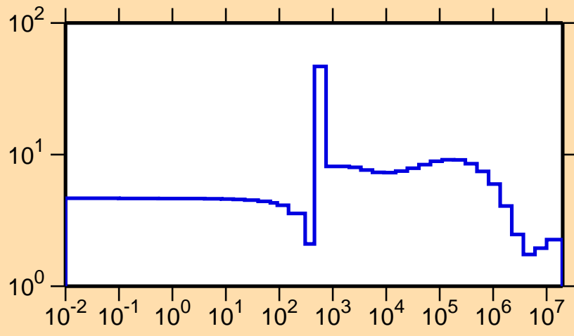
\sigma vs. E for ^{96}\text{Pd}(n,\text{el.})
