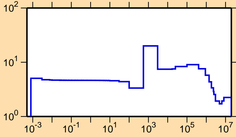
\sigma vs. E for ^{96}\text{Pd}(n,\text{el.})
