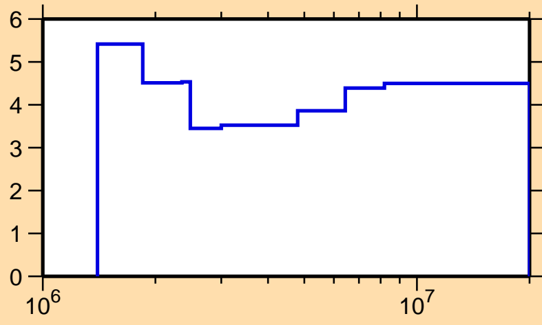
\Delta\sigma/\sigma vs. E for ^{96}\text{Pd}(n,\text{tot.})
