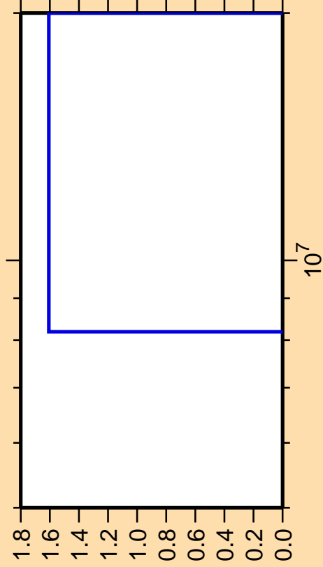
\Delta\sigma/\sigma vs. E for ^{96}\text{Pd}(n,nd)
