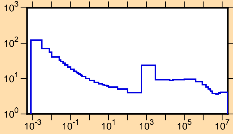
\sigma vs. E for ^{96}\text{Pd}(n,\text{tot.})
