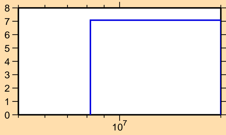
\Delta\sigma/\sigma vs. E for ^{96}\text{Pd}(n,\text{el.})
