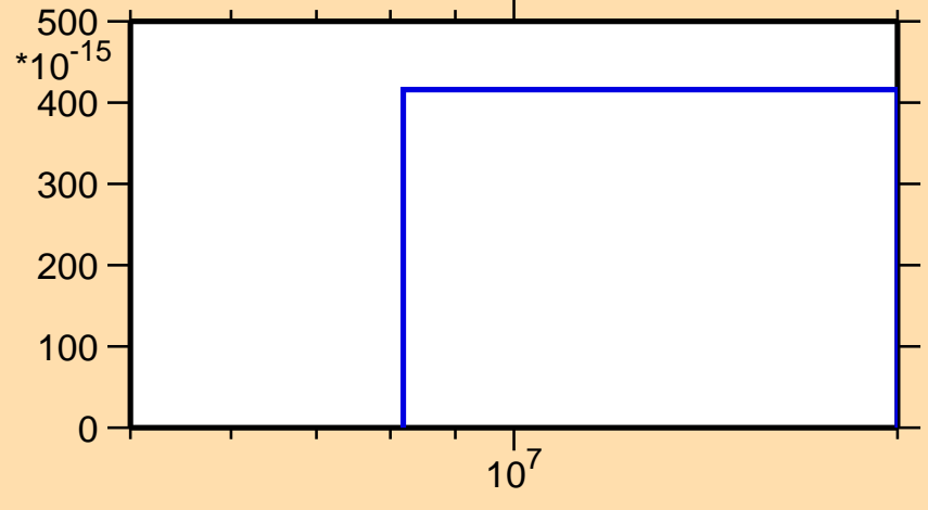
\sigma vs. E for ^{96}\text{Pd}(n,nd)
