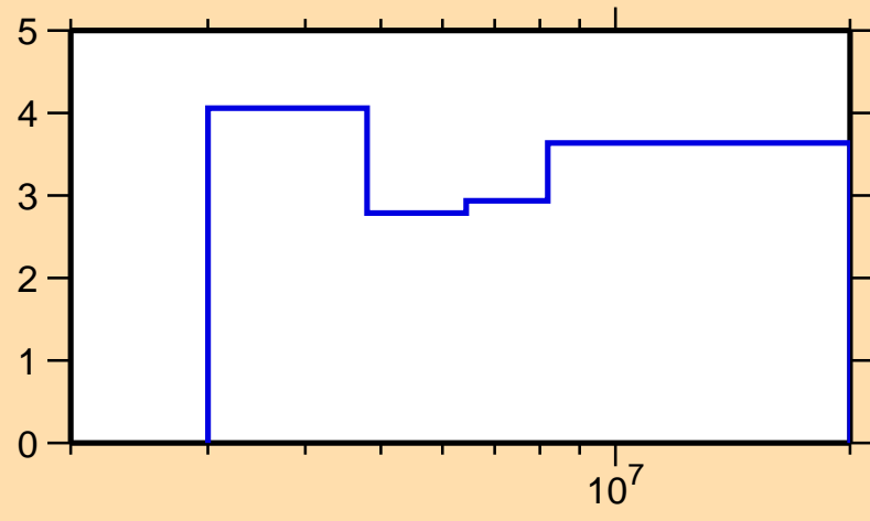
\Delta\sigma/\sigma vs. E for ^{96}\text{Pd}(n,\text{nonel.})
