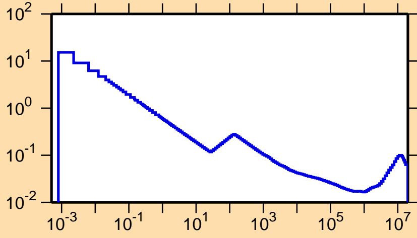
\sigma vs. E for ^{97}\text{Pd}(n,\alpha)
