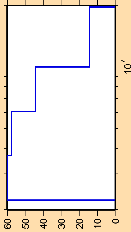
\Delta\sigma/\sigma vs. E for ^{97}\text{Pd}(n,n\text{cont.})
