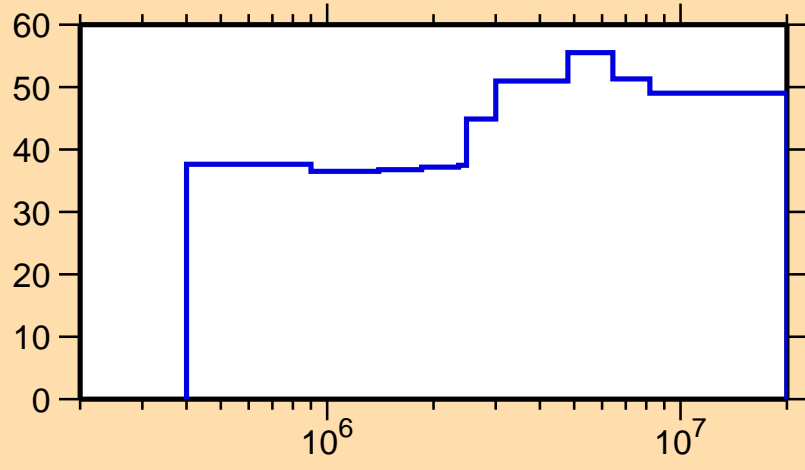
\Delta\sigma/\sigma vs. E for ^{97}\text{Pd}(n,n_1)
