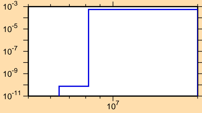
\sigma vs. E for ^{97}\text{Pd}(n,n\alpha)
