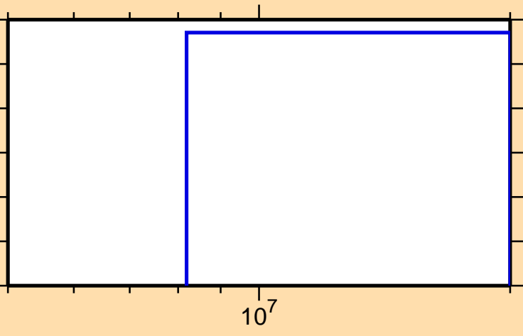
\sigma vs. E for ^{97}\text{Pd}(n,2n)
