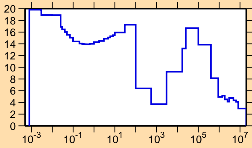
\Delta\sigma/\sigma vs. E for ^{97}\text{Pd}(n,\text{tot.})
