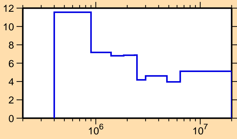
\Delta\sigma/\sigma vs. E for ^{97}\text{Pd}(n,\text{nonel.})
