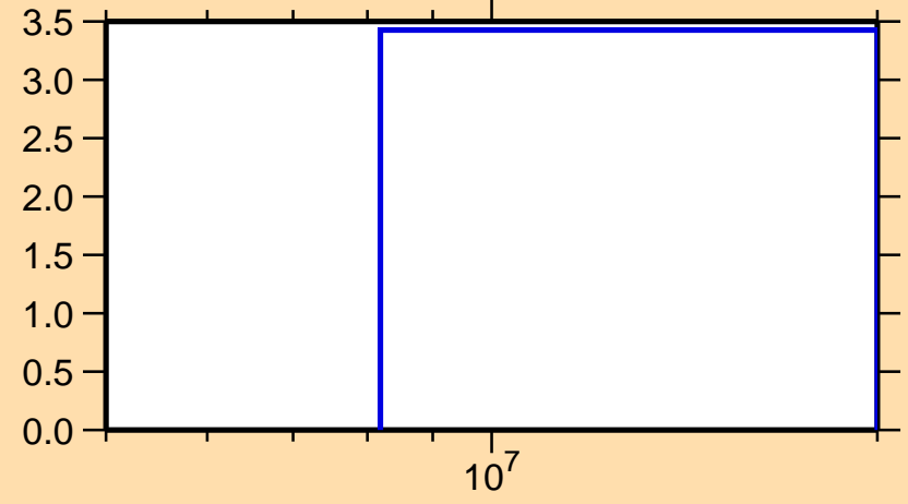
\Delta\sigma/\sigma vs. E for ^{98}\text{Pd}(n,\text{nonel.})
