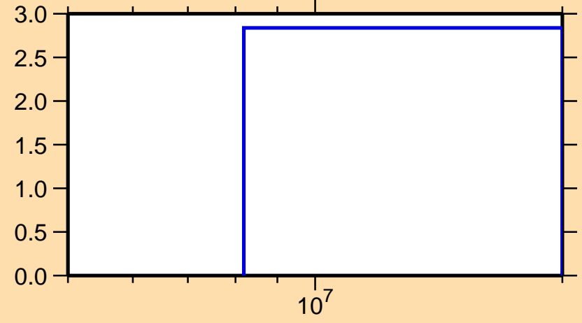
\Delta\sigma/\sigma vs. E for ^{98}\text{Pd}(n,\text{tot.})
