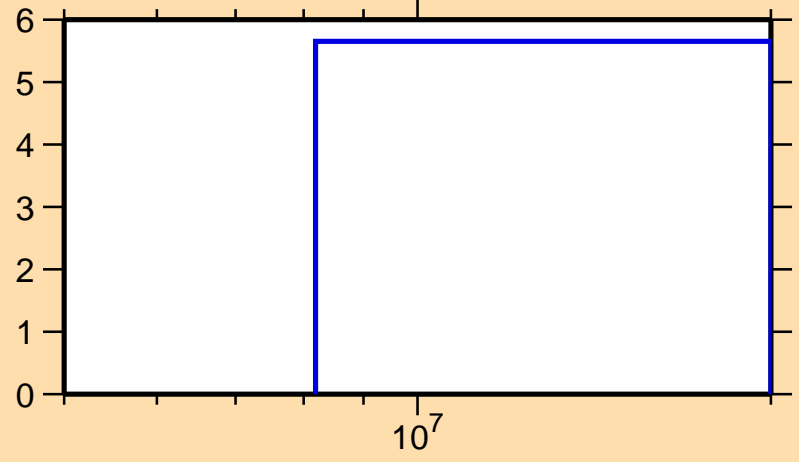
\Delta\sigma/\sigma vs. E for ^{98}\text{Pd}(n,\text{el.})
