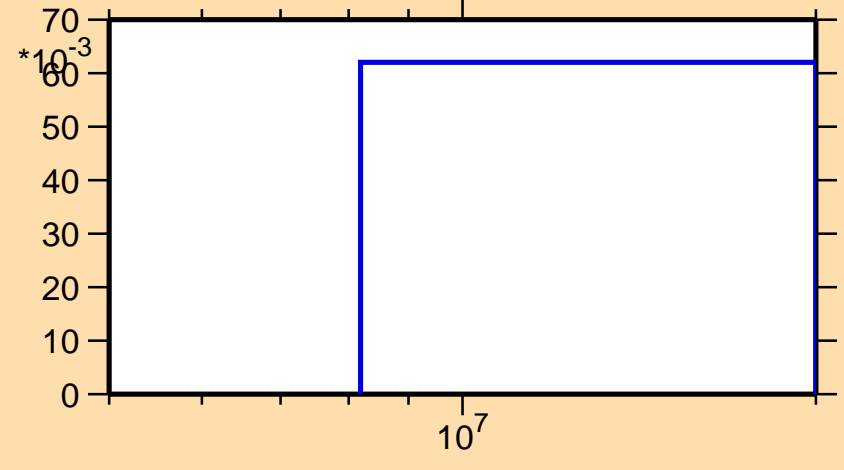
\sigma vs. E for ^{98}\text{Pd}(n,2n)
