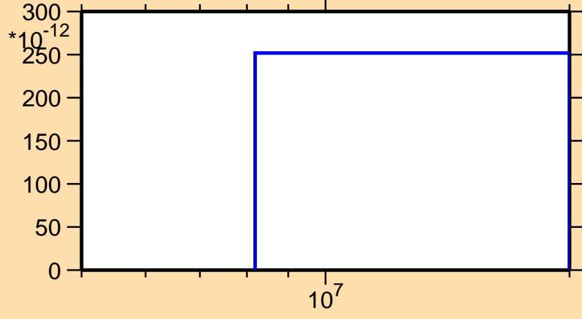
\sigma vs. E for ^{98}\text{Pd}(n,\text{pt})
