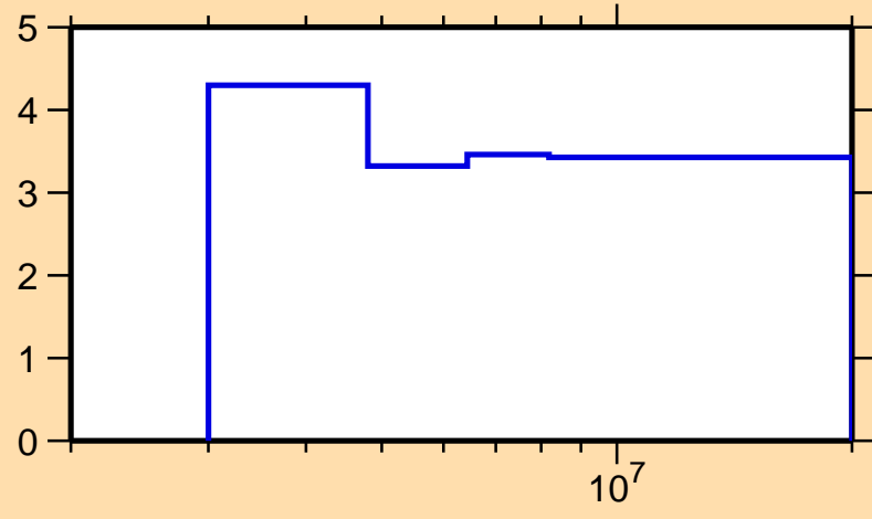
\Delta\sigma/\sigma vs. E for ^{98}\text{Pd}(n,\text{nonel.})
