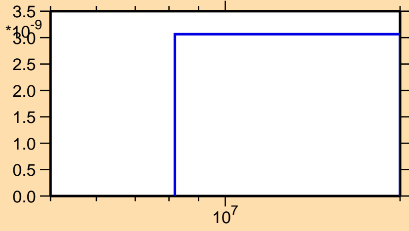
\sigma vs. E for ^{98}\text{Pd}(n,\text{nd})
