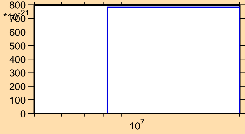
\sigma vs. E for ^{98}\text{Pd}(n,nt)
