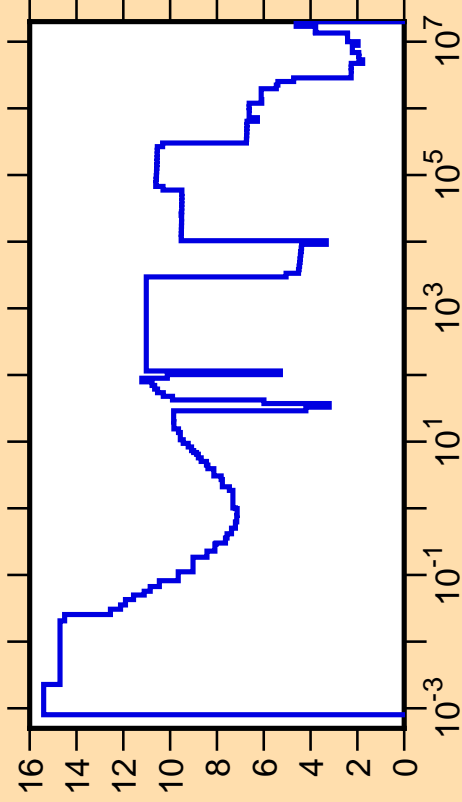
\Delta\sigma/\sigma vs. E for ^{99}\text{Pd}(n,\text{tot.})
