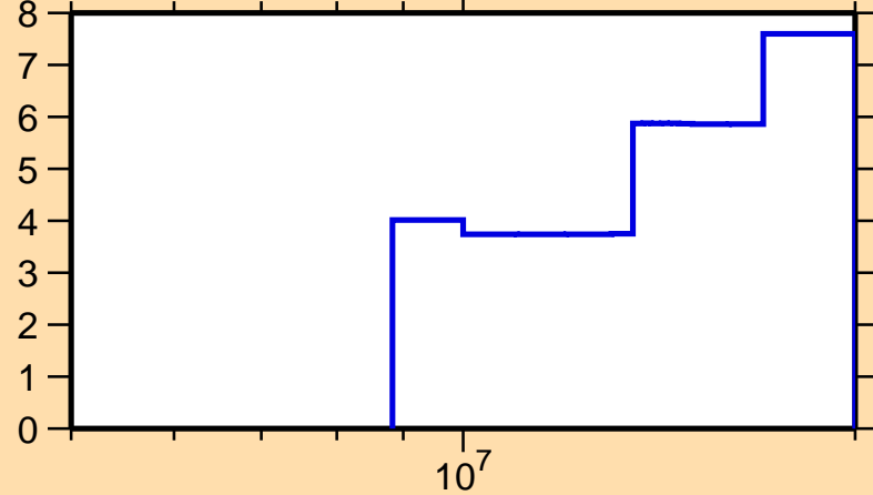
\Delta\sigma/\sigma vs. E for ^{99}\text{Pd}(n,\text{el.})
