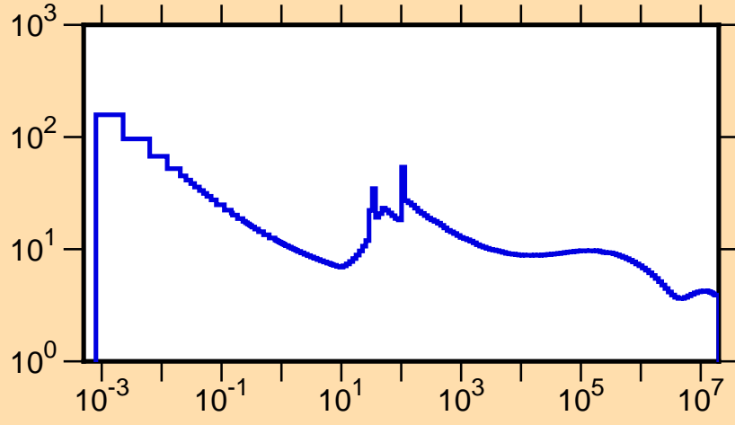
\sigma vs. E for ^{99}\text{Pd}(n,\text{tot.})
