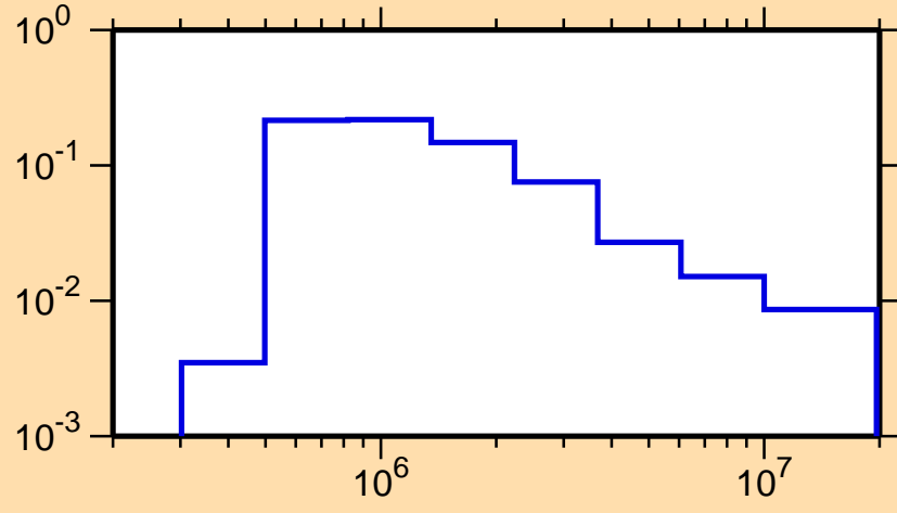
\sigma vs. E for ^{99}\text{Pd}(n,n_3)
