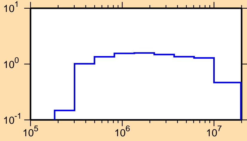
\sigma vs. E for ^{99}\text{Pd}(n,\text{inel.})
