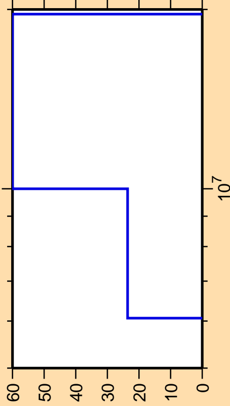
\Delta\sigma/\sigma vs. E for ^{99}\text{Pd}(n,\text{He}3)
