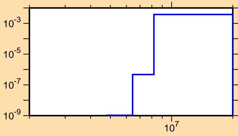
\sigma vs. E for ^{99}\text{Pd}(n,p\alpha)
