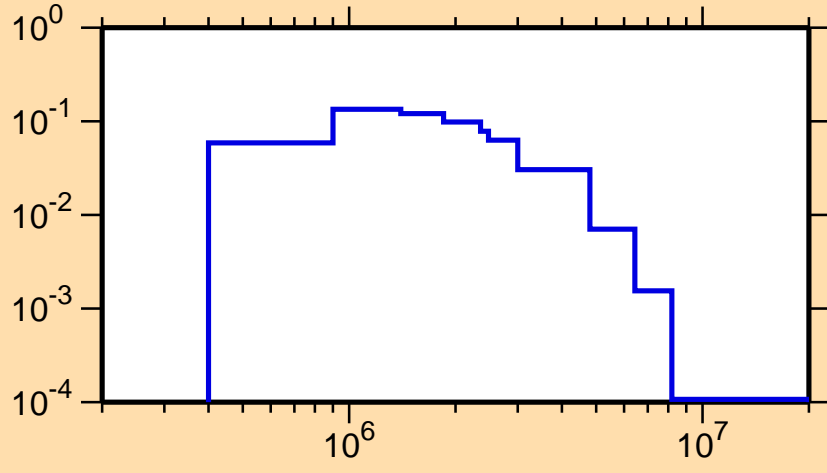
\sigma vs. E for ^{99}\text{Pd}(n,n_4)
