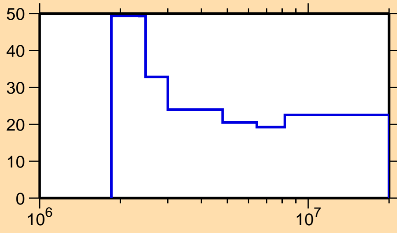
\Delta\sigma/\sigma vs. E for ^{99}\text{Pd}(n,n\text{cont.})
