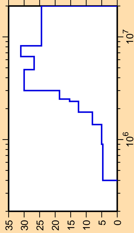
\Delta\sigma/\sigma vs. E for ^{99}\text{Pd}(n,n_4)
