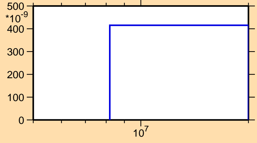
\sigma vs. E for ^{99}\text{Pd}(n,nd)
