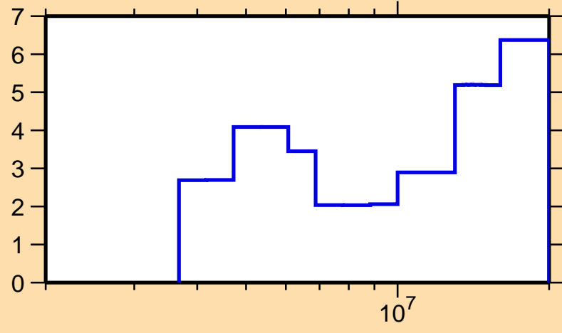
\Delta\sigma/\sigma vs. E for ^{100}\text{Pd}(n, \text{el.})
