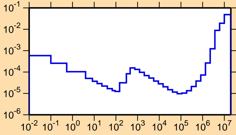
\sigma vs. E for ^{100}\text{Pd}(n,\alpha)
