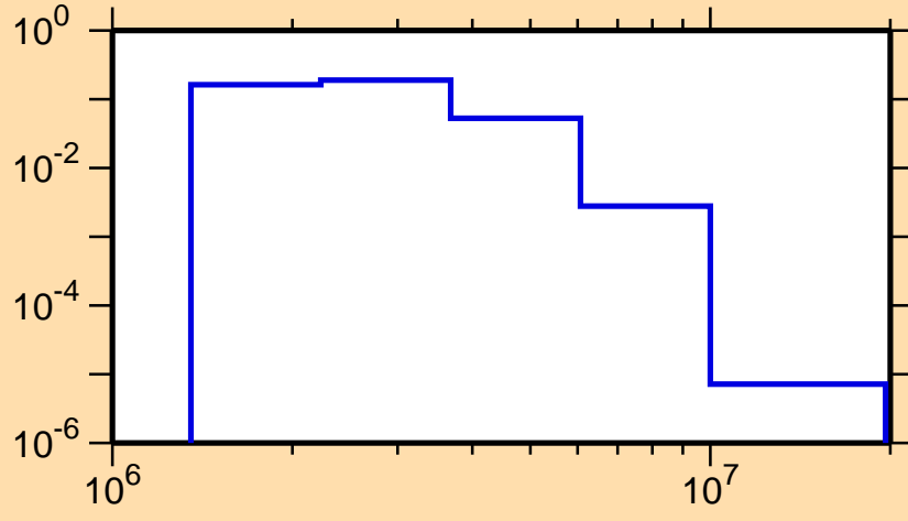
\sigma vs. E for ^{100}\text{Pd}(n,n_3)
