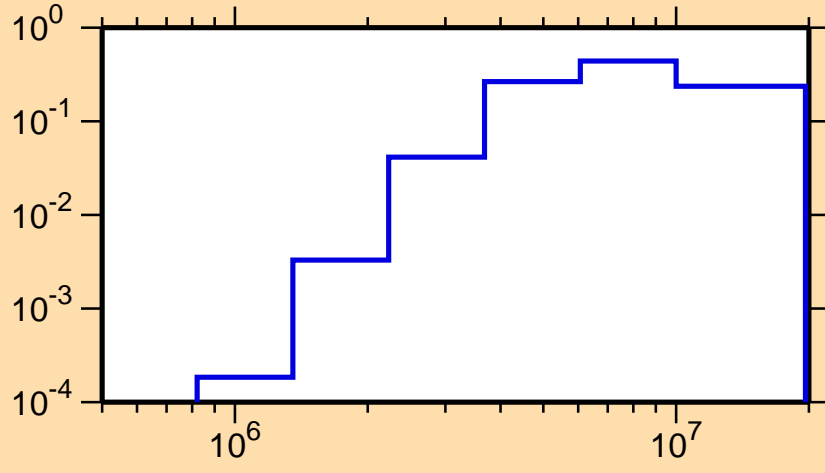
\sigma vs. E for ^{100}\text{Pd}(n,p)
