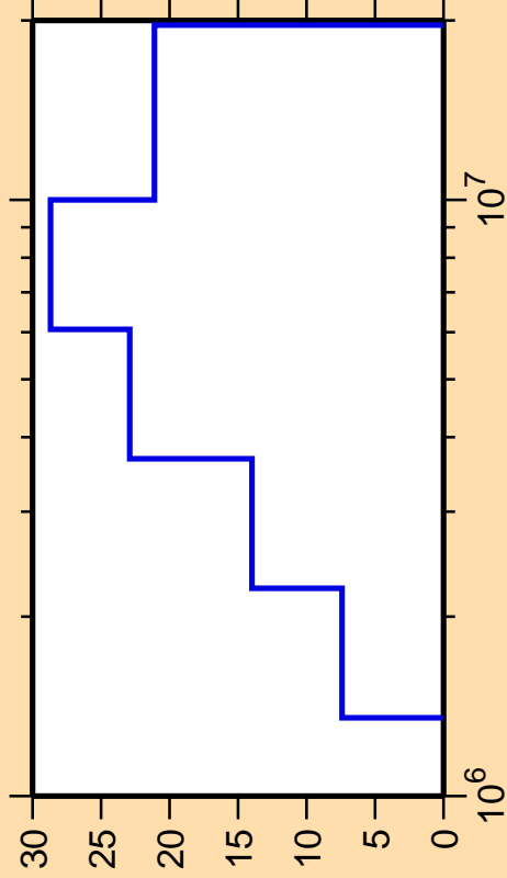
\Delta\sigma/\sigma vs. E for ^{100}\text{Pd}(n,n_3)
