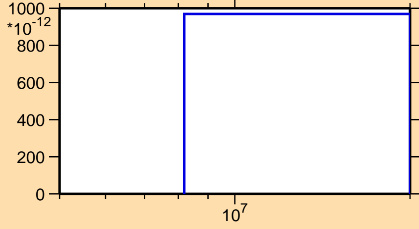
\sigma vs. E for ^{100}\text{Pd}(n,nd)
