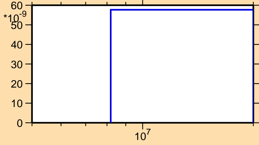
\sigma vs. E for ^{100}\text{Pd}(n,\text{pd})
