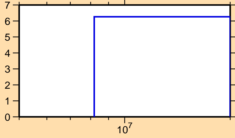
\Delta\sigma/\sigma vs. E for ^{100}\text{Pd}(n,\text{inel.})
