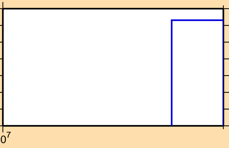
\sigma vs. E for ^{101}\text{Pd}(n,3n)
