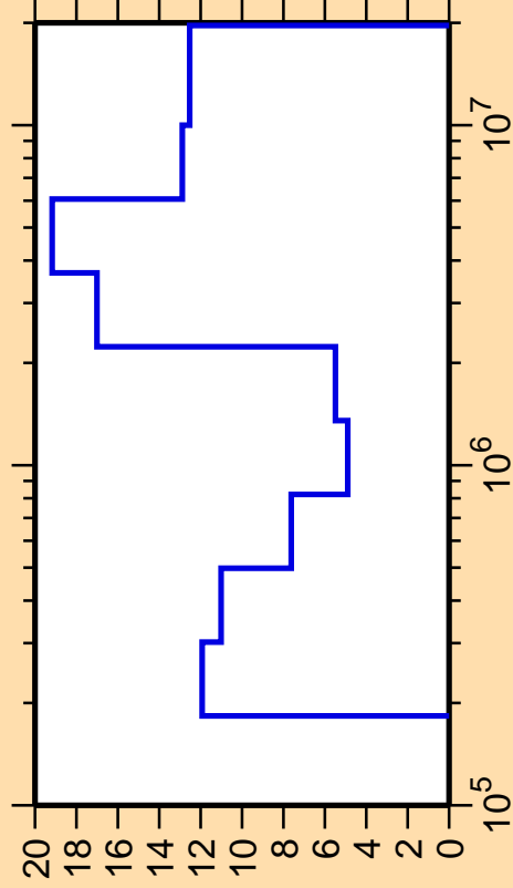
\Delta\sigma/\sigma vs. E for ^{101}\text{Pd}(n,n_2)
