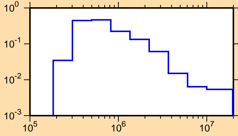
\sigma vs. E for ^{101}\text{Pd}(n,n_2)
