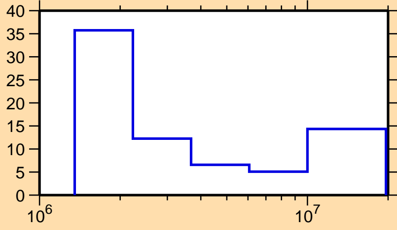
\Delta\sigma/\sigma vs. E for ^{101}\text{Pd}(n,n\text{cont.})
