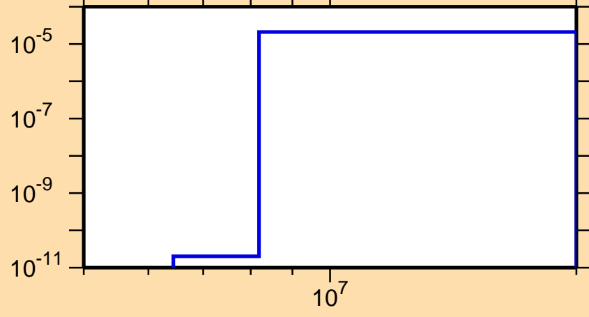
\sigma vs. E for ^{101}\text{Pd}(n,p\alpha)
