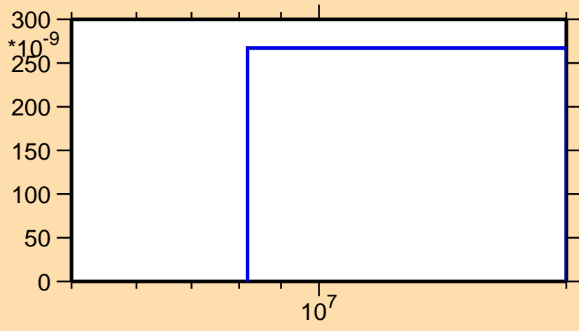
\sigma vs. E for ^{101}\text{Pd}(n,\text{He}3)
