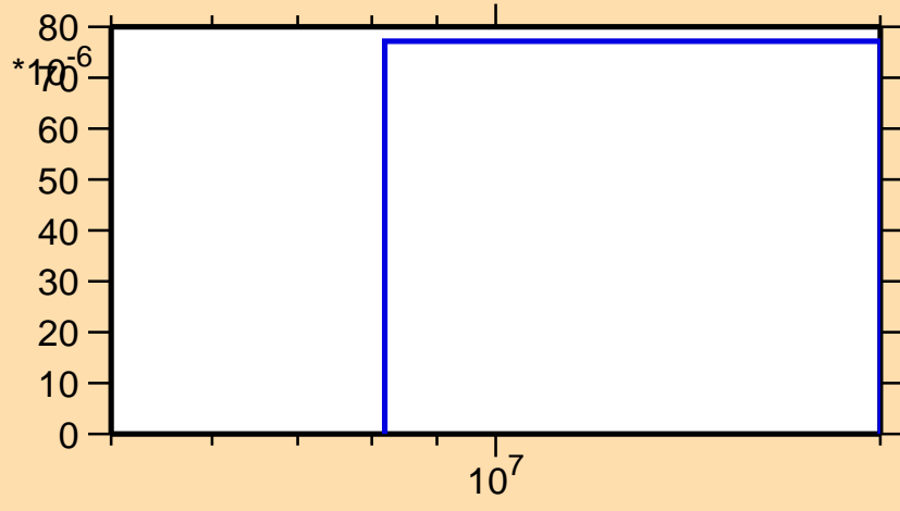
\sigma vs. E for ^{101}\text{Pd}(n,t)
