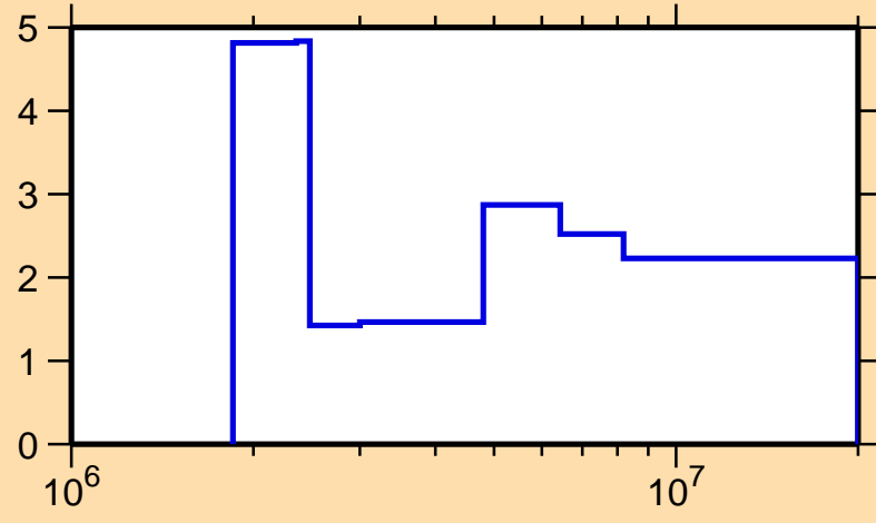
\Delta\sigma/\sigma vs. E for ^{101}\text{Pd}(n,\text{el.})
