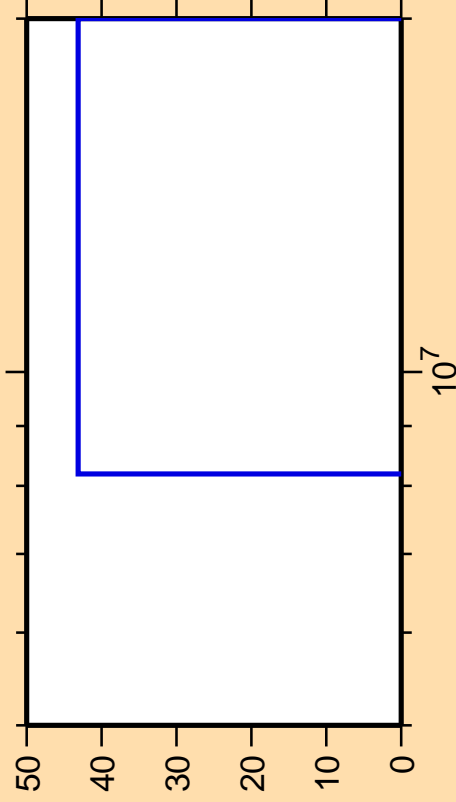
\Delta\sigma/\sigma vs. E for ^{101}\text{Pd}(n,nd)
