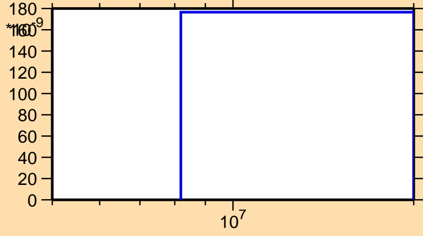
\sigma vs. E for ^{101}\text{Pd}(n,nd)
