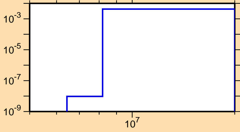
\sigma vs. E for ^{101}\text{Pd}(n,d)
