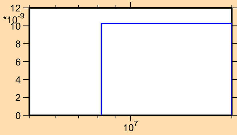
\sigma vs. E for ^{101}\text{Pd}(n,3n)
