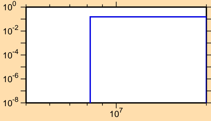
\sigma vs. E for ^{101}\text{Pd}(n,np)
