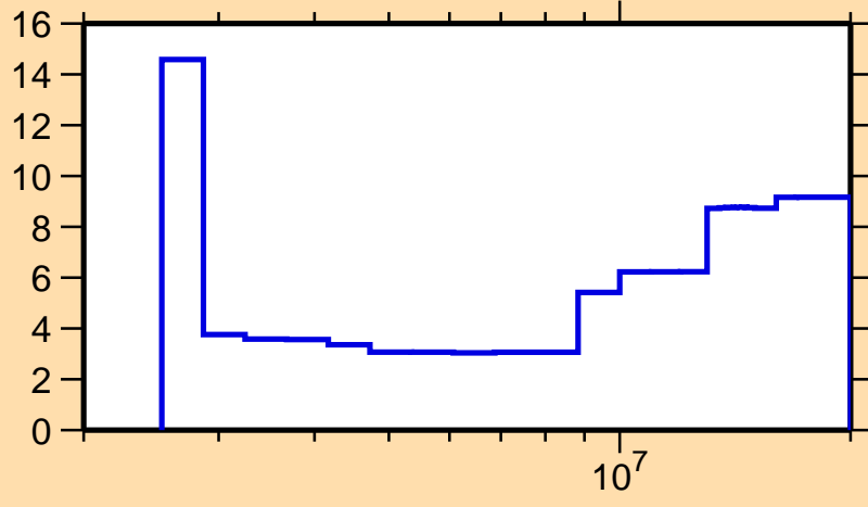
\Delta\sigma/\sigma vs. E for ^{102}\text{Pd}(n,n\text{cont.})
