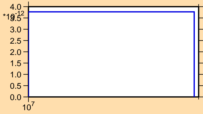
\sigma vs. E for ^{102}\text{Pd}(n,2np)
