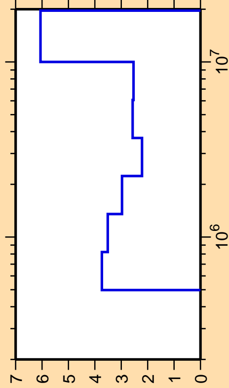
\Delta\sigma/\sigma vs. E for ^{102}\text{Pd}(n,\text{inel.})
