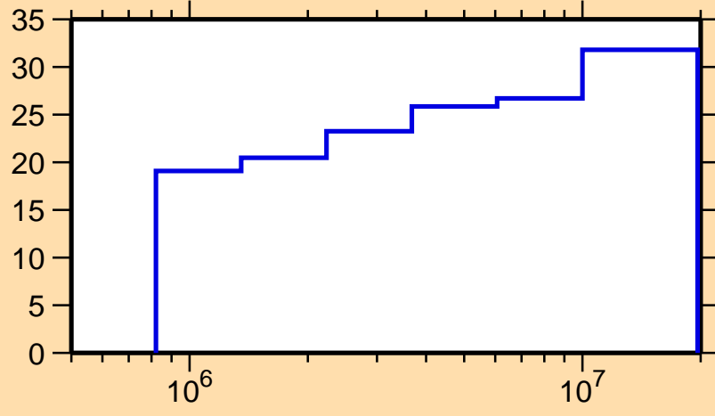
\Delta\sigma/\sigma vs. E for ^{102}\text{Pd}(n,\gamma)
