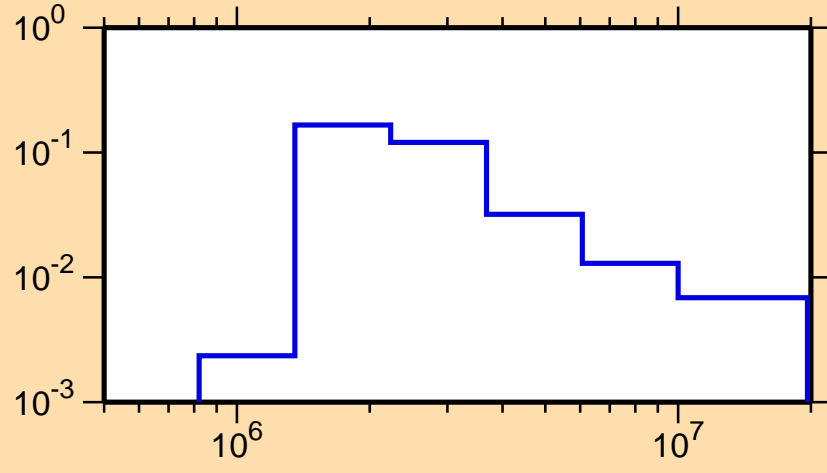
\sigma vs. E for ^{102}\text{Pd}(n,n_2)
