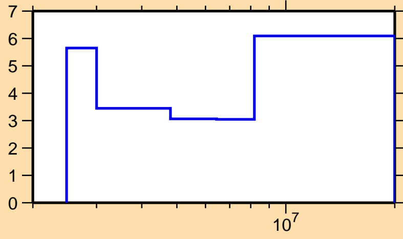
\Delta\sigma/\sigma vs. E for ^{102}\text{Pd}(n,n\text{cont.})
