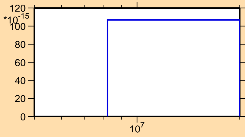
\sigma vs. E for ^{102}\text{Pd}(\text{mt117})
