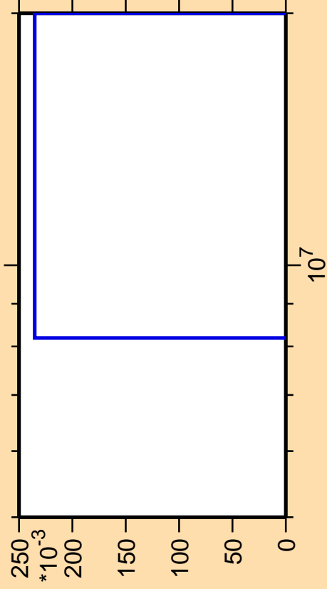
\Delta\sigma/\sigma vs. E for ^{102}\text{Pd}(\text{mt117})
