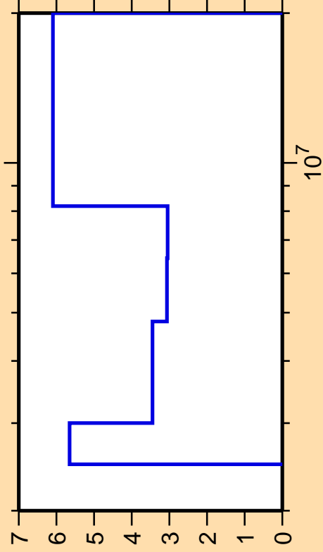
\Delta\sigma/\sigma vs. E for ^{102}\text{Pd}(n,n\text{cont.})
