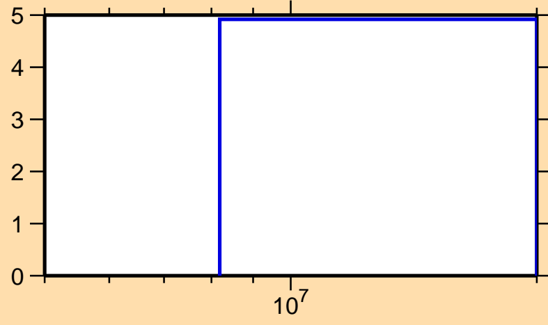
\Delta\sigma/\sigma vs. E for ^{102}\text{Pd}(n,\text{inel.})
