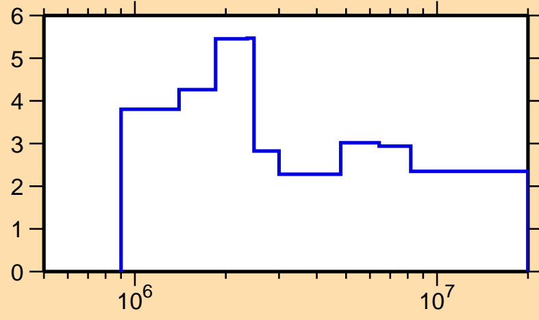
\Delta\sigma/\sigma vs. E for ^{102}\text{Pd}(n,\text{el.})
