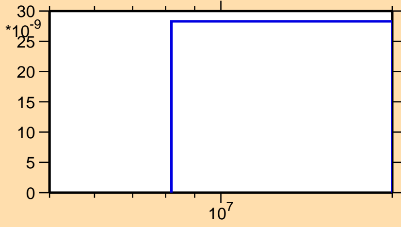
\sigma vs. E for ^{102}\text{Pd}(n,p\alpha)
