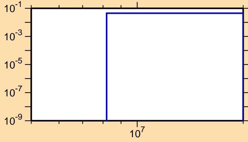
\sigma vs. E for ^{102}\text{Pd}(n,np)
