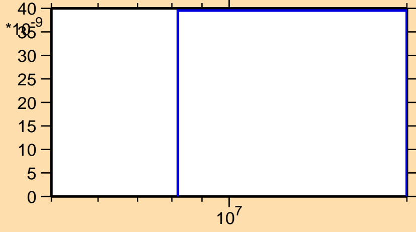
\sigma vs. E for ^{102}\text{Pd}(n,\text{He}3)
