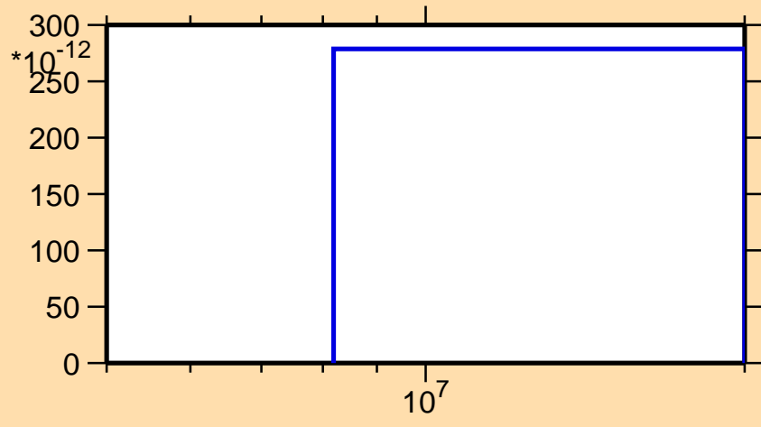
\sigma vs. E for ^{102}\text{Pd}(n,\text{pd})
