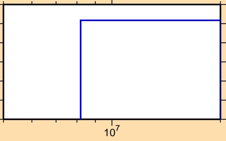
\sigma vs. E for ^{103}\text{Pd}(n,\text{He}3)
