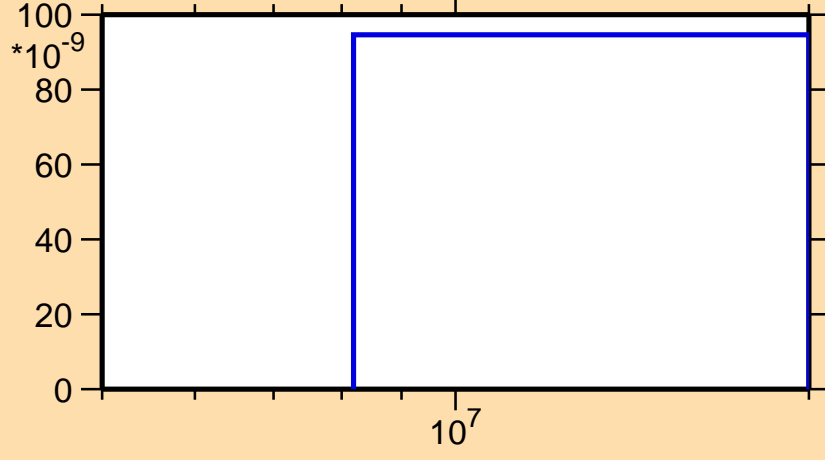
\sigma vs. E for ^{103}\text{Pd}(n,p\alpha)
