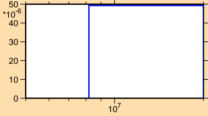
\sigma vs. E for ^{103}\text{Pd}(n,t)
