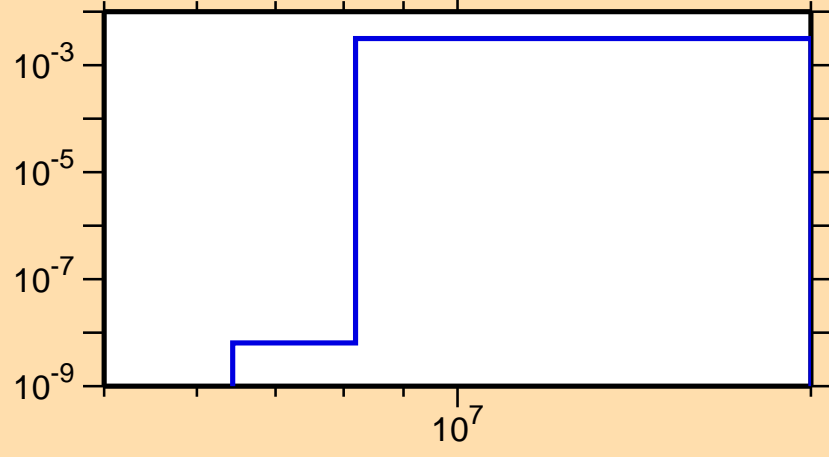
\sigma vs. E for ^{103}\text{Pd}(n,n\alpha)
