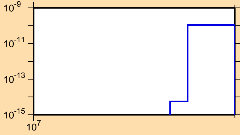
\sigma vs. E for ^{104}\text{Pd}(n,\text{pd})
