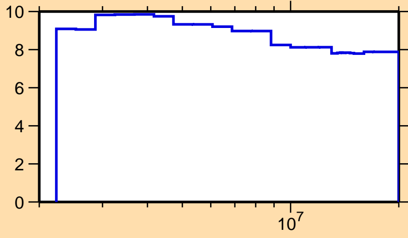
\Delta\sigma/\sigma vs. E for ^{104}\text{Pd}(n, n_1)
