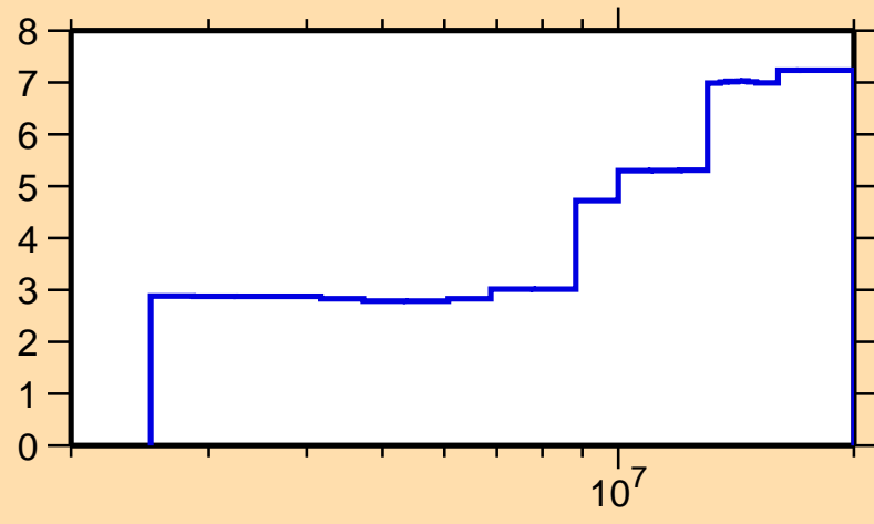
\Delta\sigma/\sigma vs. E for ^{104}\text{Pd}(n,n\text{cont.})
