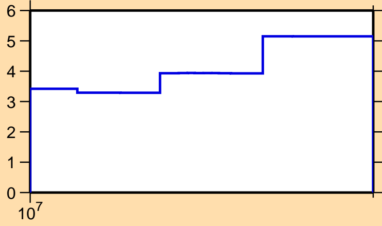
\Delta\sigma/\sigma vs. E for ^{104}\text{Pd}(n, 2n)
