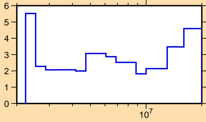
\Delta\sigma/\sigma vs. E for ^{104}\text{Pd}(n, \text{el.})
