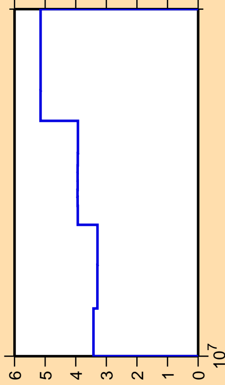
\Delta\sigma/\sigma vs. E for ^{104}\text{Pd}(n,2n)
