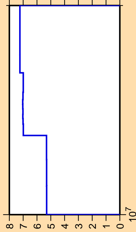
\Delta\sigma/\sigma vs. E for ^{104}\text{Pd}(n, n_{\text{cont}})
