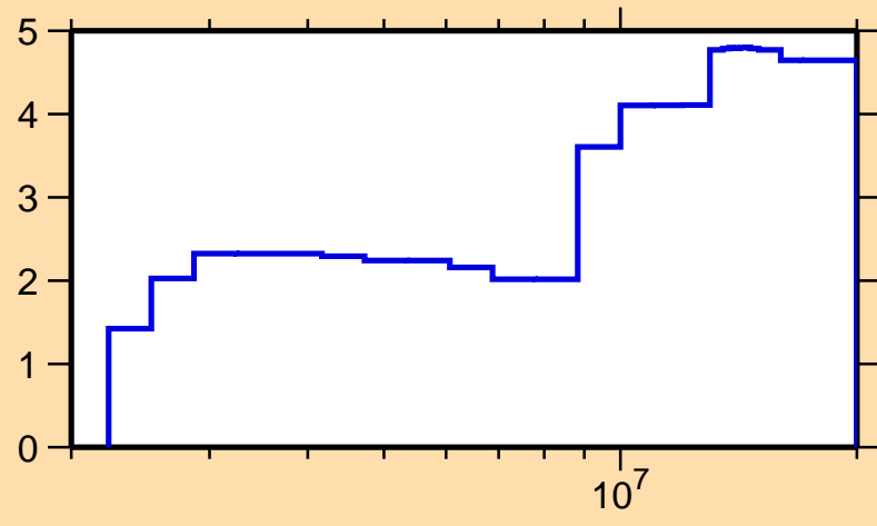
\Delta\sigma/\sigma vs. E for ^{104}\text{Pd}(n,\text{inel.})
