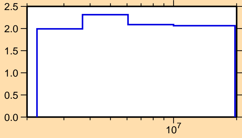
\Delta\sigma/\sigma vs. E for ^{104}\text{Pd}(n,n\text{onel.})
