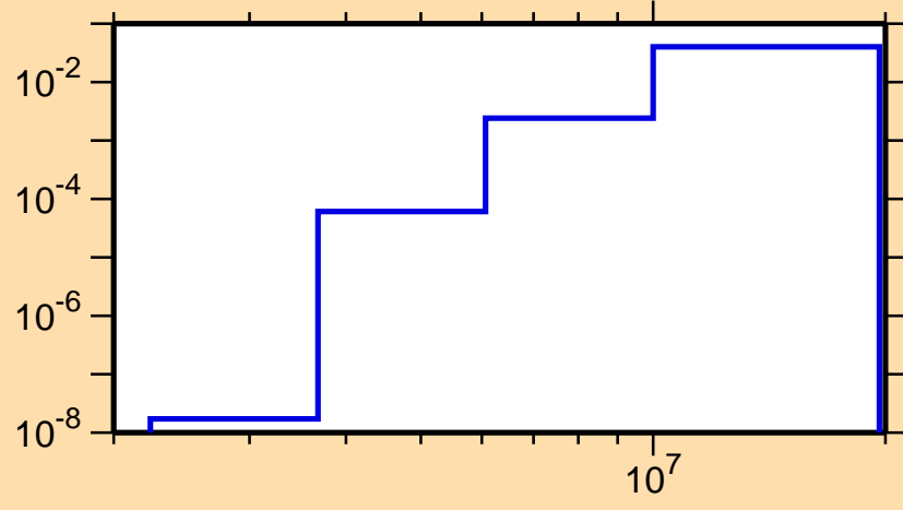
\sigma vs. E for ^{104}\text{Pd}(n,p)
