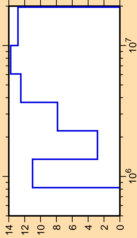
\Delta\sigma/\sigma vs. E for ^{104}\text{Pd}(n,n_2)
