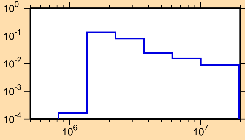
\sigma vs. E for ^{104}\text{Pd}(n,n_2)
