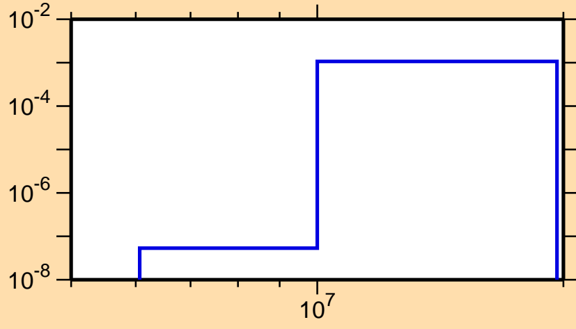
\sigma vs. E for ^{104}\text{Pd}(n,n\alpha)
