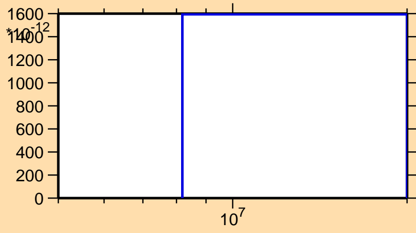
\sigma vs. E for ^{105}\text{Pd}(n,\text{He}3)
