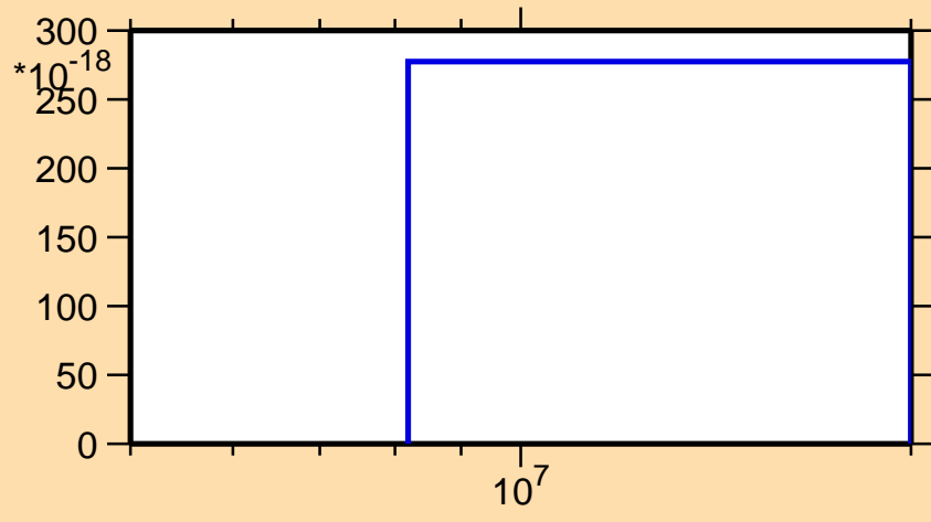
\sigma vs. E for ^{105}\text{Pd}(n,\text{pd})
