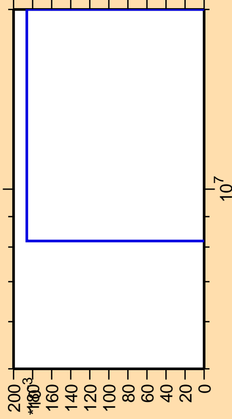
\Delta\sigma/\sigma vs. E for ^{105}\text{Pd}(n,nt)
