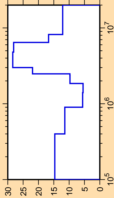
\Delta\sigma/\sigma vs. E for ^{105}\text{Pd}(n,n_2)
