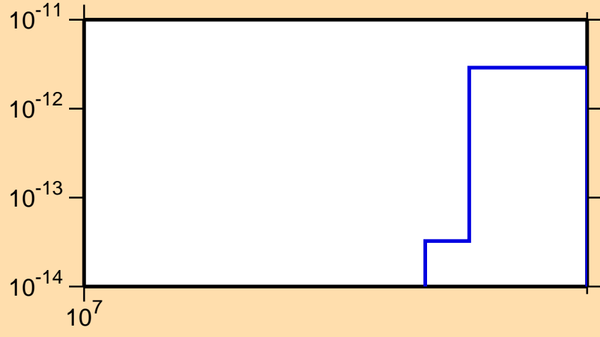
\sigma vs. E for ^{106}\text{Pd}(n,p\alpha)
