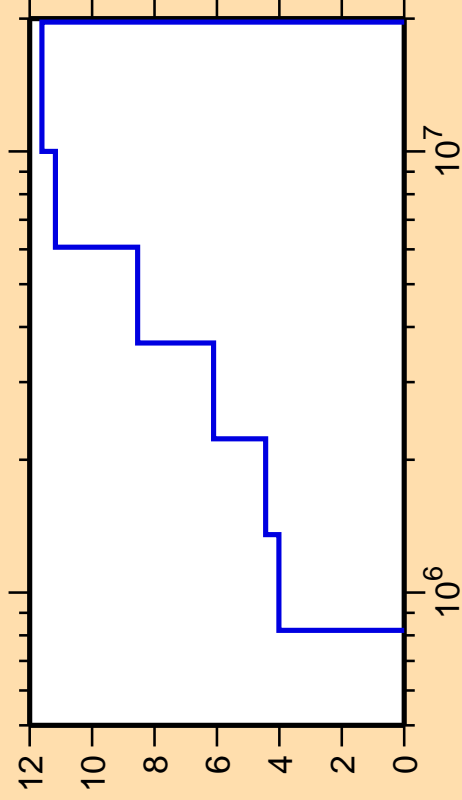
\Delta\sigma/\sigma vs. E for ^{106}\text{Pd}(n,n_2)
