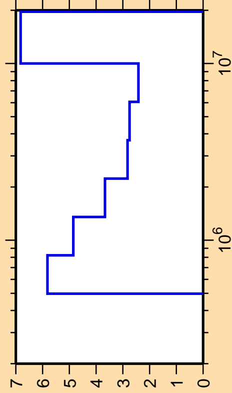
\Delta\sigma/\sigma vs. E for ^{106}\text{Pd}(n,\text{inel.})
