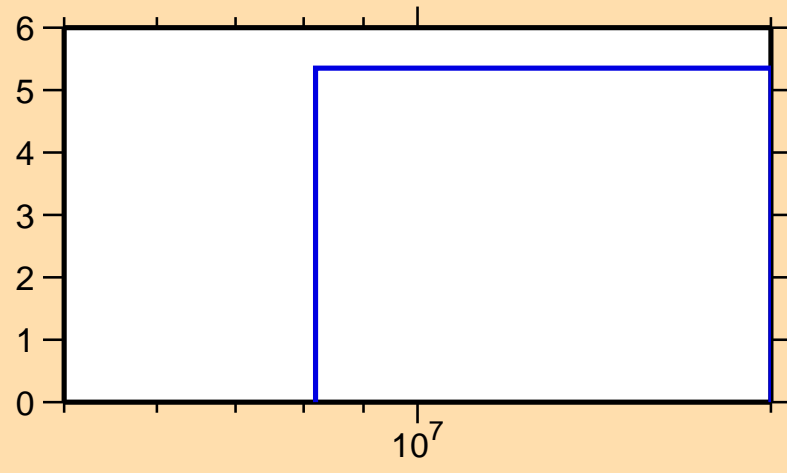
\Delta\sigma/\sigma vs. E for ^{106}\text{Pd}(n,\text{inel.})
