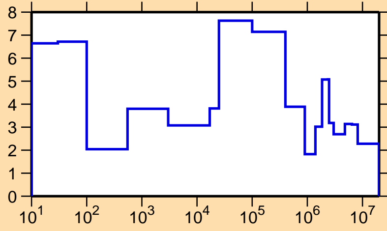
\Delta\sigma/\sigma vs. E for ^{106}\text{Pd}(n,\text{el.})
