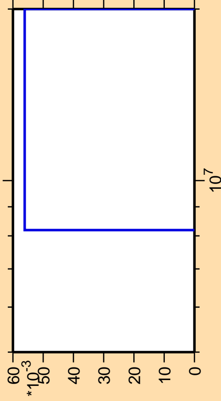
\Delta\sigma/\sigma vs. E for ^{106}\text{Pd}(n,nt)
