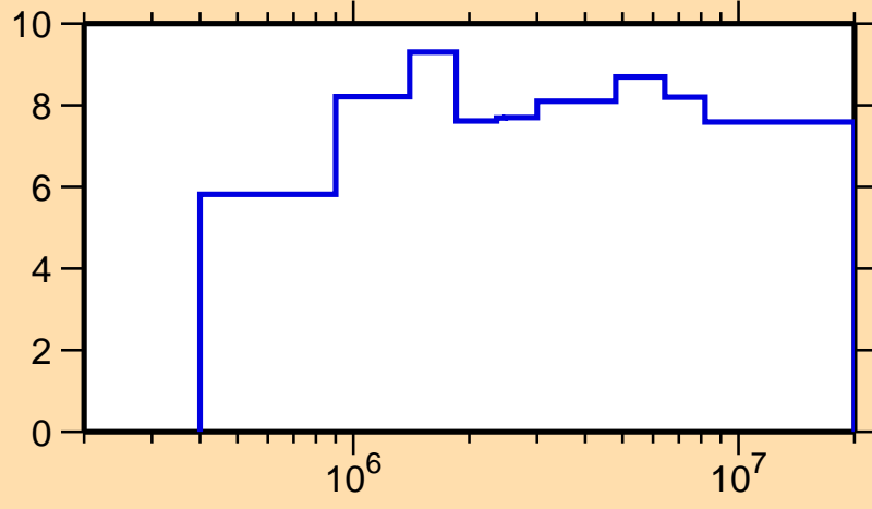
\Delta\sigma/\sigma vs. E for ^{106}\text{Pd}(n,n_1)
