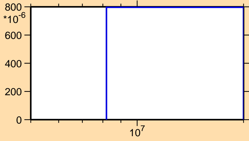
\sigma vs. E for ^{106}\text{Pd}(n,d)
