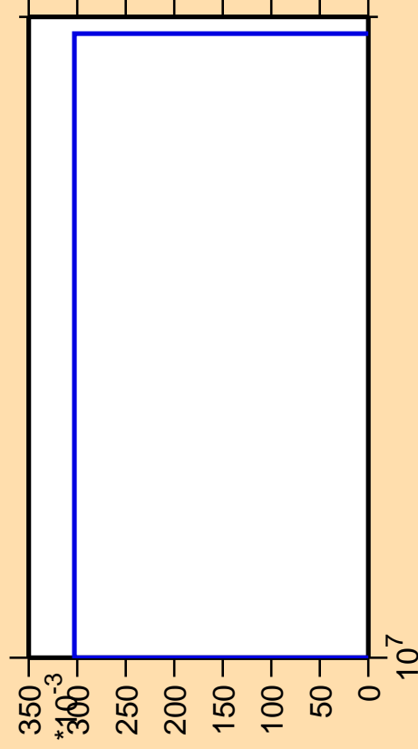
\Delta\sigma/\sigma vs. E for ^{107}\text{Pd}(n,nt)
