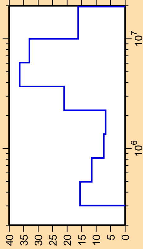
\Delta\sigma/\sigma vs. E for ^{107}\text{Pd}(n,n_4)
