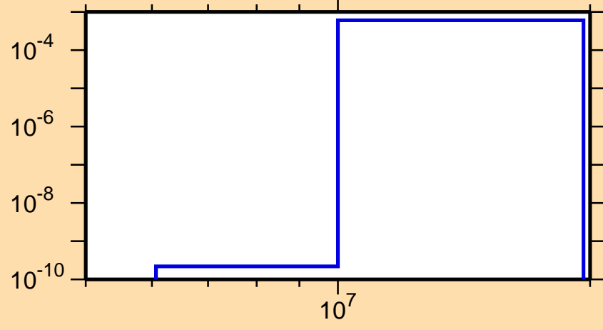
\sigma vs. E for ^{107}\text{Pd}(n,n\alpha)
