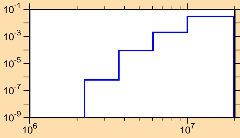
\sigma vs. E for ^{107}\text{Pd}(n,p)
