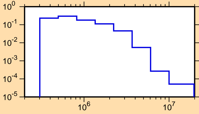
\sigma vs. E for ^{107}\text{Pd}(n,n_4)
