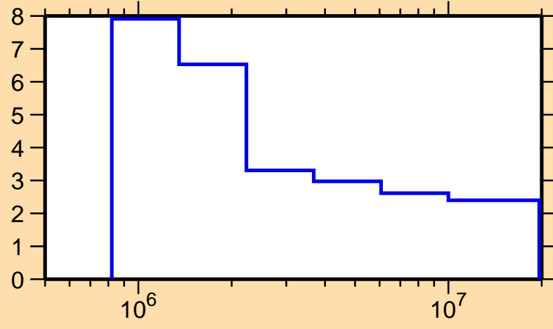
\Delta\sigma/\sigma vs. E for ^{107}\text{Pd}(n, n_{\text{onel}})
