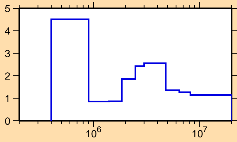
\Delta\sigma/\sigma vs. E for ^{107}\text{Pd}(n, tot.)
