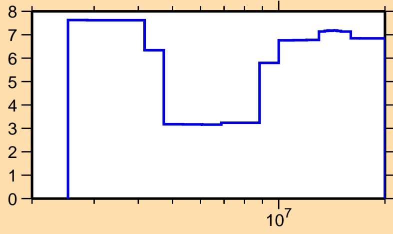
\Delta\sigma/\sigma vs. E for ^{108}\text{Pd}(n,n\text{cont.})
