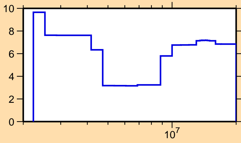
\Delta\sigma/\sigma vs. E for ^{108}\text{Pd}(n,n\text{cont.})
