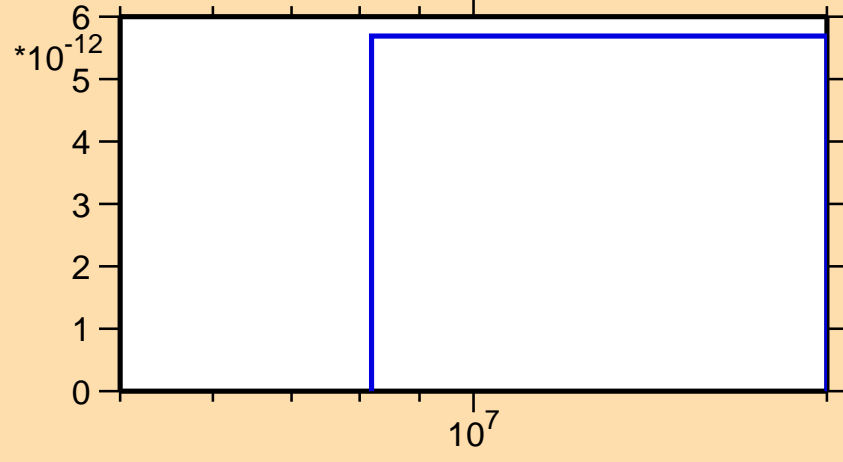
\sigma vs. E for ^{108}\text{Pd}(n,nd)
