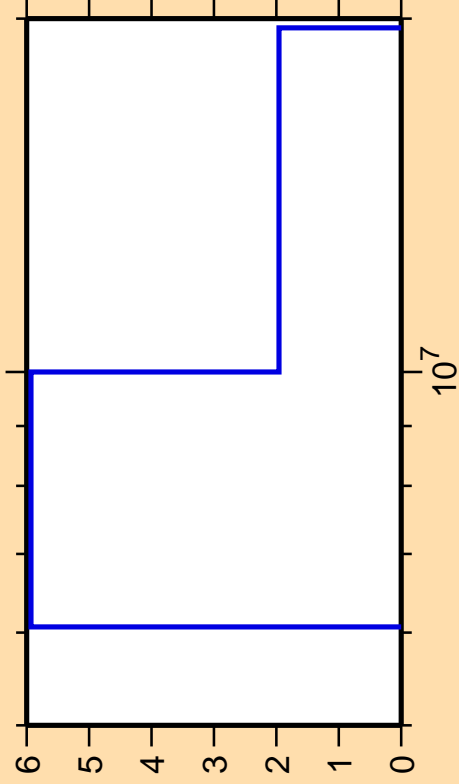
\Delta\sigma/\sigma vs. E for ^{109}\text{Pd}(n,2n)
