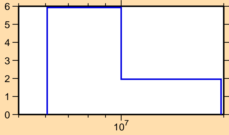
\Delta\sigma/\sigma vs. E for ^{109}\text{Pd}(n,2n)
