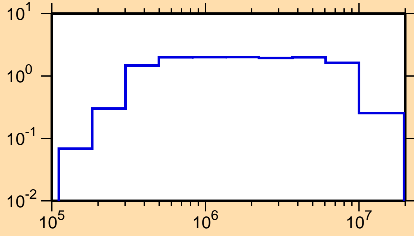
\sigma vs. E for ^{109}\text{Pd}(n,\text{inel.})
