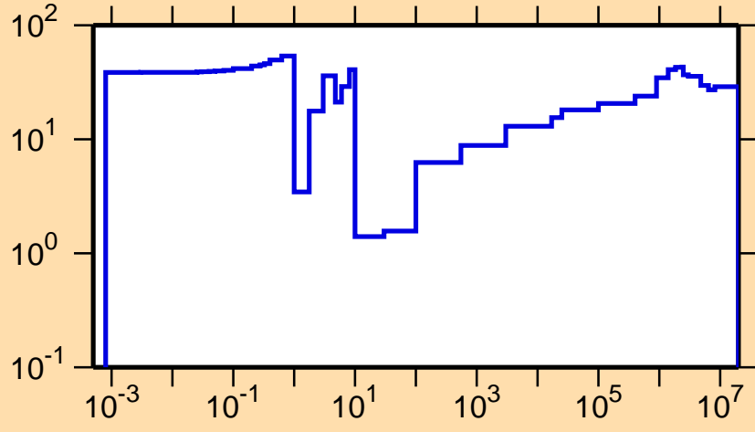
\Delta\sigma/\sigma vs. E for ^{109}\text{Pd}(n,\gamma)
