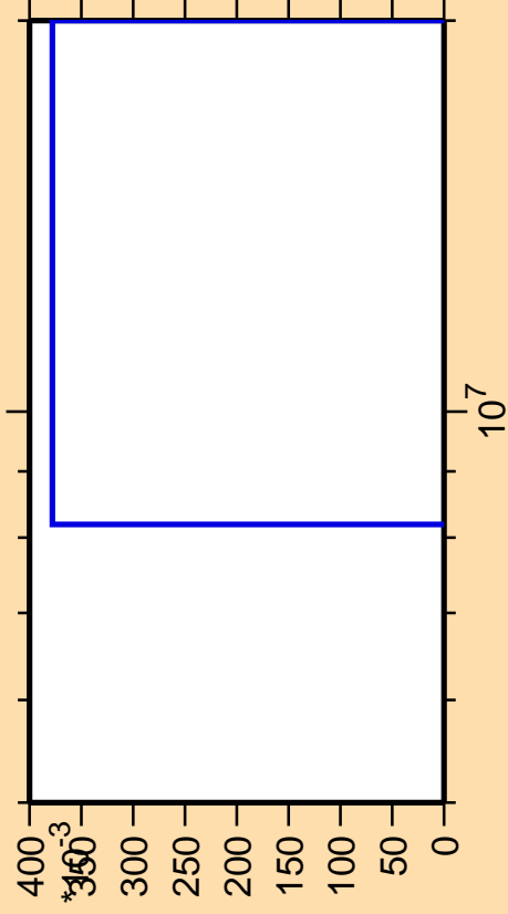
\Delta\sigma/\sigma vs. E for ^{109}\text{Pd}(n,\text{He}3)
