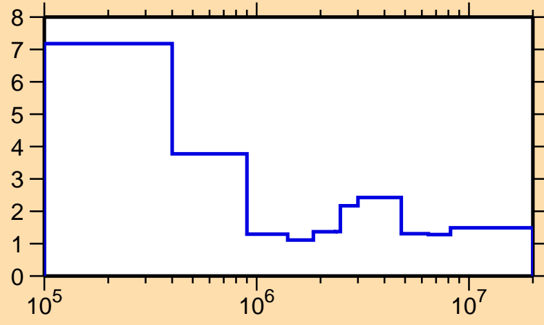
\Delta\sigma/\sigma vs. E for ^{109}\text{Pd}(n,\text{tot.})
