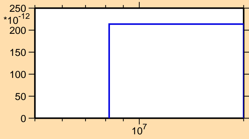
\sigma vs. E for ^{109}\text{Pd}(n,2n\alpha)
