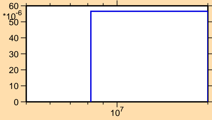
\sigma vs. E for ^{109}\text{Pd}(n,n\alpha)
