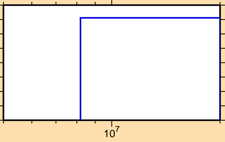
\sigma vs. E for ^{109}\text{Pd}(n,np)
