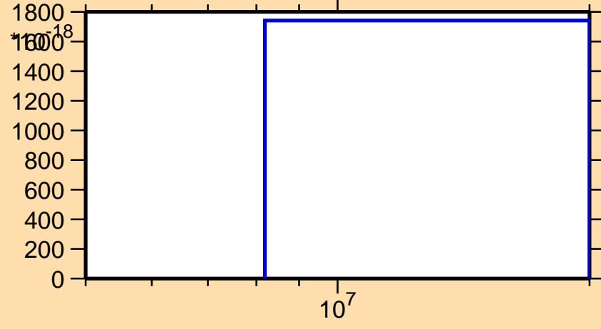
\sigma vs. E for ^{109}\text{Pd}(n,p\alpha)
