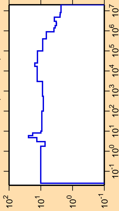
\Delta\sigma/\sigma vs. E for ^{109}\text{Pd}(n,\text{nonel.})
