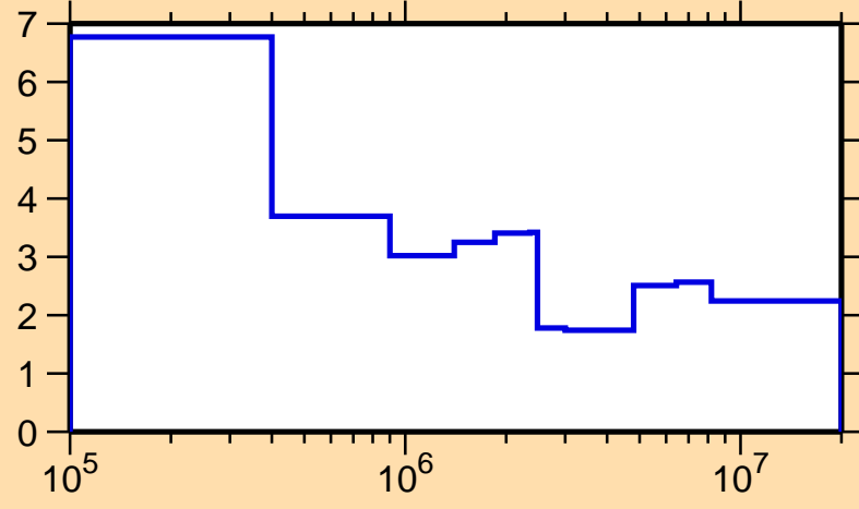
\Delta\sigma/\sigma vs. E for ^{109}\text{Pd}(n,\text{el.})
