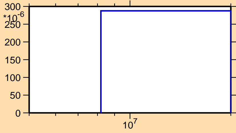
\sigma vs. E for ^{109}\text{Pd}(n,d)
