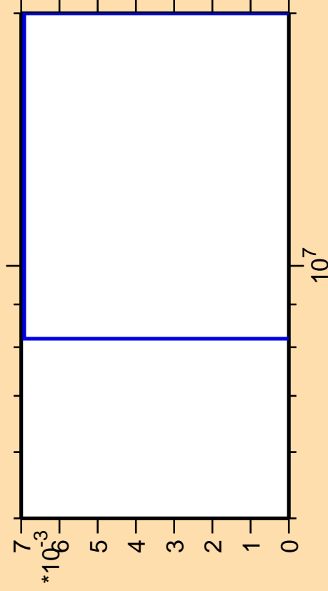
\Delta\sigma/\sigma vs. E for ^{109}\text{Pd}(n,p\alpha)
