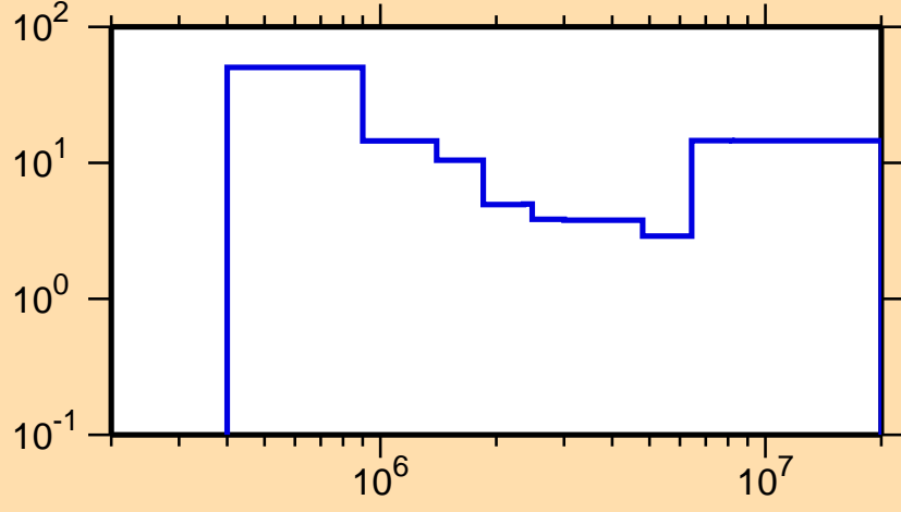
\Delta\sigma/\sigma vs. E for ^{109}\text{Pd}(n,n\text{cont.})
