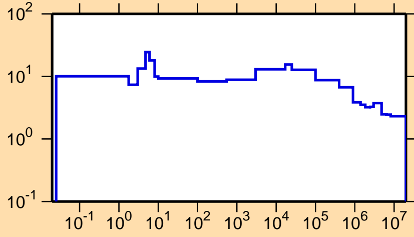
\Delta\sigma/\sigma vs. E for ^{109}\text{Pd}(n,\text{nonel.})
