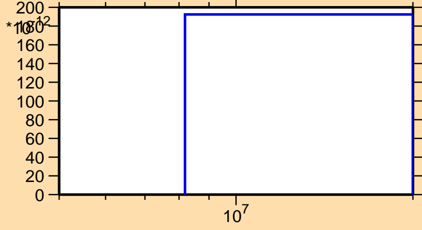
\sigma vs. E for ^{109}\text{Pd}(n,2np)
