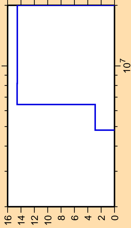
\Delta\sigma/\sigma vs. E for ^{109}\text{Pd}(n,n\text{cont.})
