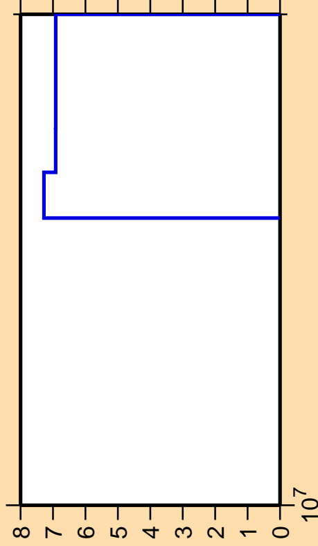
\Delta\sigma/\sigma vs. E for ^{109}\text{Pd}(n,3n)
