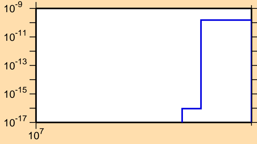
\sigma vs. E for ^{109}\text{Pd}(n,nt)
